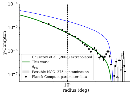
Figure 24. Comparison between the Compton parameter profile measured by Planck and that inferred from our thermal model. We also show the result of the extrapolation of the model by [153].
