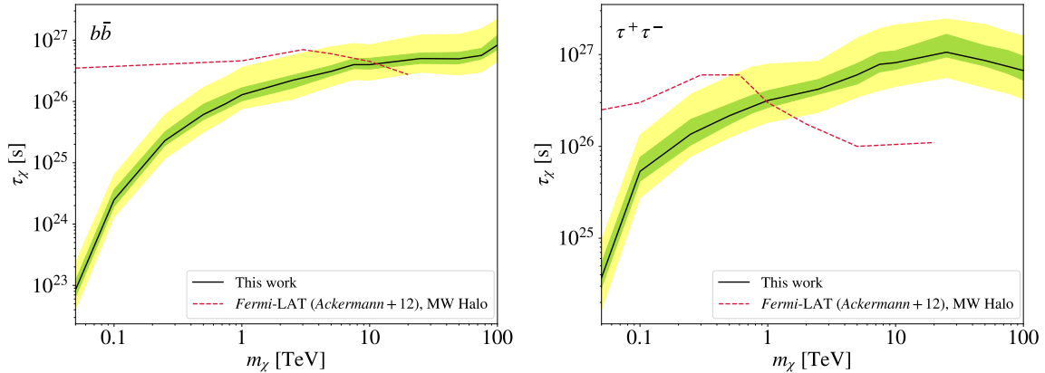
Figure 22. 95% C.L. mean lower limits of the lifetime of the DM particle versus the DM mass (black lines) for b\bar{b} (left panel) and \tau^+\tau^- (right panel) decay channels, in comparison with the limits obtained by [227] (corresponding to NFW 5\sigma free source fits, in dashed red lines). The green (yellow) band shows the 1\sigma ( 2\sigma ) scatter of the projected limits. All of our results are shown for the template fitting analysis, unless stated otherwise.
