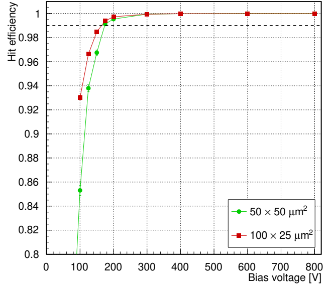
Figure 21: Hit efficiency for normal beam incidence as a function of bias voltage for sensors with pixel sizes of 50 \times 50 \text{ μm}^2 (R4S50x50-P1) and 100 \times 25 \text{ μm}^2 (R4S100x25-P1). Both sensors were irradiated with protons to a fluence of \Phi_{\text{eq}} = 2.4 \times 10^{15} \text{ cm}^{-2} .
