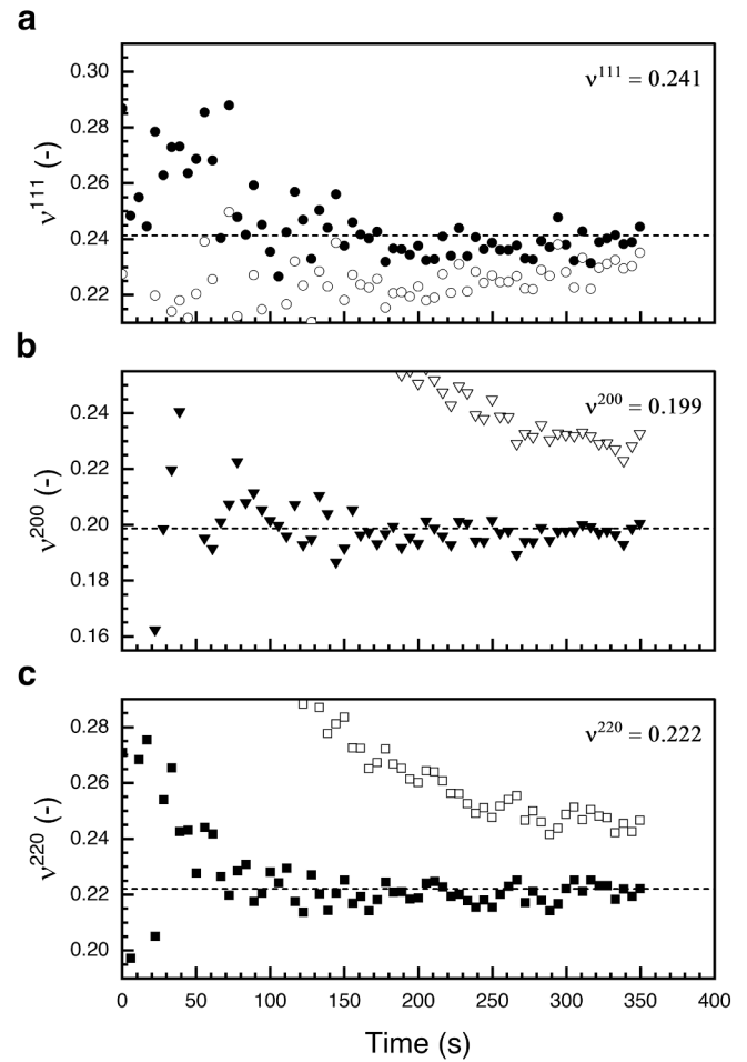
Fig. 5. Poisson's ratio values of \text{Ti}_{0.8}\text{B}_{0.2} obtained for three crystallographic plane families {111}, {200}, and {220} shown in panels (a) circular symbols, (b) triangular symbols, and (c) square symbols, respectively. The dashed horizontal line in each panel represents the \nu^{hkl} value calculated from the negative ratio of the slope of the lateral and axial strain components, as indicated in the upper right corner. All framed symbols denote the initial \nu_{d_0}^{hkl} values calculated pointwise from the negative ratio of \epsilon_{yy}^{hkl} and \epsilon_{zz}^{hkl} , while filled symbols show the least squares fitted \nu_{d_0,r}^{hkl} values after iterative “fminsearch” (a derivative-free minimization routine of MATLAB) optimization of the strain-free lattice parameter from d_0^{hkl} to d_{0,r}^{hkl} . Notably, certain initial \nu_{d_0}^{hkl} values deviate strongly from the \nu^{hkl} target value and appear (not visible) outside the plot.
