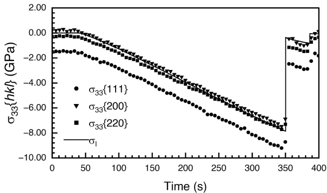
Fig. 6. Uniaxial compressive stress analysis of a \text{TiN}_{0.2}\text{B}_{0.8} micropillar showing the stress components evaluated for \{111\} (circular symbols), \{200\} (triangular symbols), and \{220\} (square symbols) evaluated for the three crystallographic planes along with the continuous stress measurements from the indenter, \sigma_I (continuous line). The plot illustrates stress evolution over load time to failure at 350 s and -7.86 GPa.
