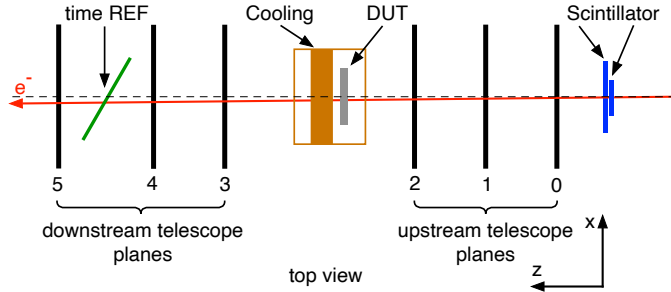
Figure 11: Sketch of the setup used for the test beam measurements, seen from the top. The time reference plane is labeled "time REF", and DUT indicates the device under test.
