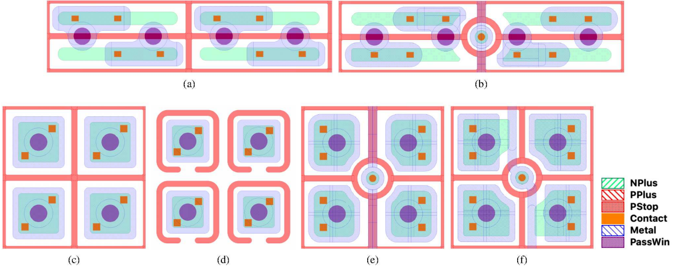
Figure 4: Mask layouts of example designs ( 100 \times 25 \mu\text{m}^2 cells in the top row and 50 \times 50 \mu\text{m}^2 cells in the bottom row) for the RD53A chip with p -stop isolation: a) Default, no bias scheme (RD53A100x25-P1). b) Common punch-through and straight bias rail (RD53A100x25-P2). c) Default, no bias scheme (RD53A 50x50-P1). d) Open p -stop (RD53A50x50-P2). e) Common punch-through and straight bias rail (RD53A50x50-P3). f) Common punch-through and wiggle bias rail (RD53A50x50-P4). The color code indicates the various mask layers: n^+ implant (NPlus), p^+ implant (PPlus), p -stop implant (PStop), metal contact via (Contact), metallization (Metal), opening in the passivation (PassWin).
