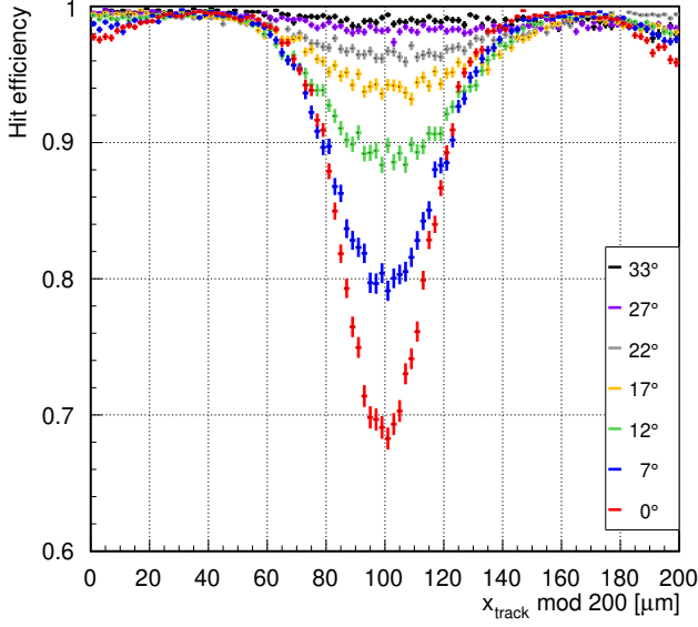
Figure 22: Hit efficiency as a function of the position inside two pixels along the 100 \mu\text{m} direction for various track angles measured at a bias voltage of 800 V. The track angle is defined with respect to the perpendicular to the sensor plane. The inclination is in the 100 \mu\text{m} direction. The measured sensor is of type RD53A100x25-P2 read out by a RD53A readout chip. The sensor was irradiated with protons to a fluence of \Phi_{\text{eq}} = 5.6 \times 10^{15} \text{ cm}^{-2} .
