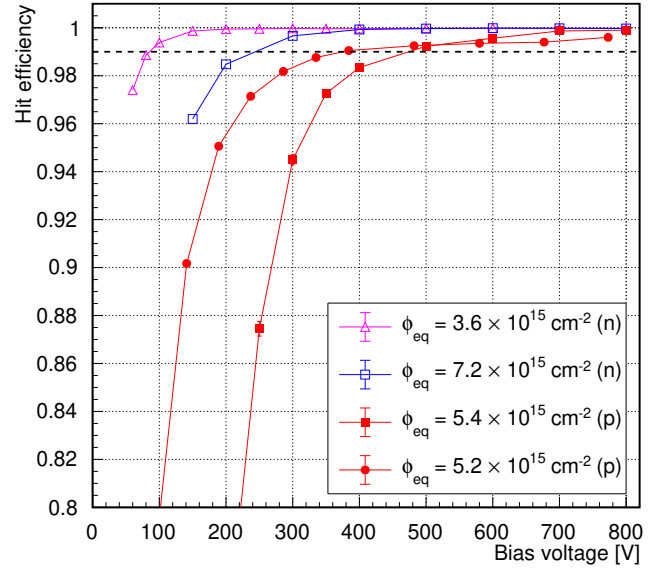
Figure 18: Hit efficiency measured at normal beam incidence as a function of bias voltage for sensors irradiated with protons (p) and neutrons (n). All ROC4Sens modules are measured at -24^\circ C . The sensors with \Phi_{eq} = 5.2 and 5.4 \times 10^{15} cm^{-2} are irradiated with protons. The sensor with 5.2 \times 10^{15} cm^{-2} (red circles) is bump bonded to a RD53A chip and measured at approximately the same temperature as the ROC4Sens modules.
