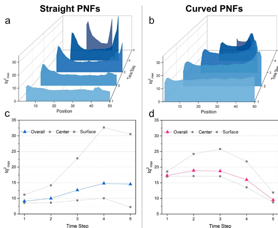
Figure 2. Maximum of the Lorentz-corrected SAXS intensity I_{q_{\max}}^2 against scanning position at different time steps during droplet drying at 40 °C for (a) straight and (b) curved PNFs. Averaged I_{q_{\max}}^2 over all of the positions, with 10% of the positions closest to the center and 10% of the positions closest to the surfaces of a drying fiber for (c) straight and (d) curved PNFs.
