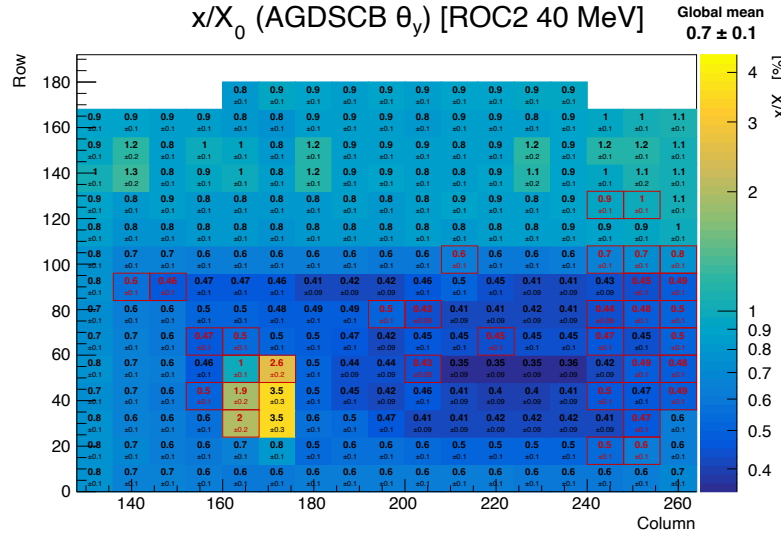
Figure 14. Fractional radiation length map of ROC2 at 40 MeV for all three fitting methods, and the combined value. Empty subregions were not fitted due to insufficient statistics, and subregions outlined in red did not meet the quality criteria for inclusion in the combined measurement. The colour axis is identical for all methods.
