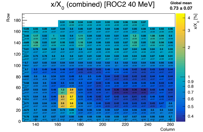
Figure 14. Fractional radiation length map of ROC2 at 40 MeV for all three fitting methods, and the combined value. Empty subregions were not fitted due to insufficient statistics, and subregions outlined in red did not meet the quality criteria for inclusion in the combined measurement. The colour axis is identical for all methods.
