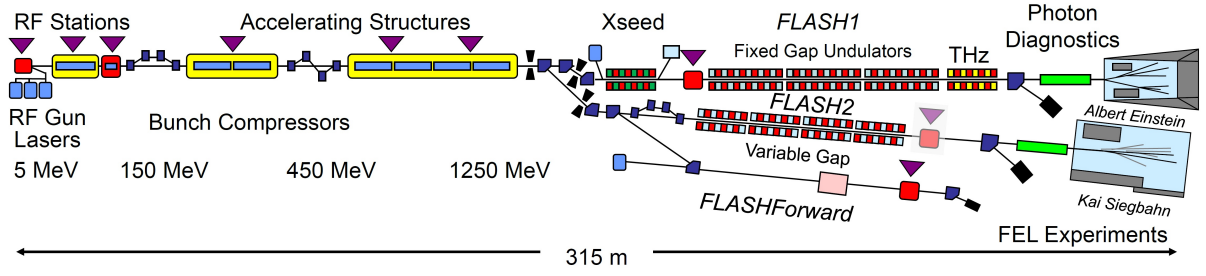
FIG. 7. Layout of the FLASH facility.
