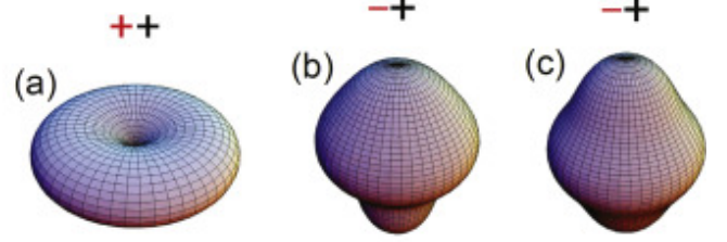
FIG. 23. PADs of the ATI of the inner 1s shell of neon for a XUV photon energy of 2 \text{ keV} and an optical (NIR) photon energy of 1.5 \text{ eV} . The helicity of the beams is indicated on top of each representation. (a) and (b) include the first-order non-dipole corrections, whereas panel (c) shows the PAD under the dipole approximation. The figure has been adapted from [181]
