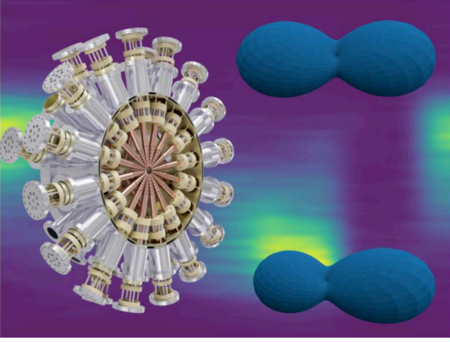
FIG. 20. Illustration of polarization characterization from streaked electron spectra. Left: CAD drawing of a new dual-interaction-plane time-of-flight apparatus for atto-streaking. The background shows angle-resolved data from the first angular streaking campaign at European XFEL from June 2022. The insets on the right illustrate the 3-dimensional angular distribution patterns for (top) linear FEL polarization of unstreaked electrons versus (bottom) electrons streaked by a circularly polarized laser.
