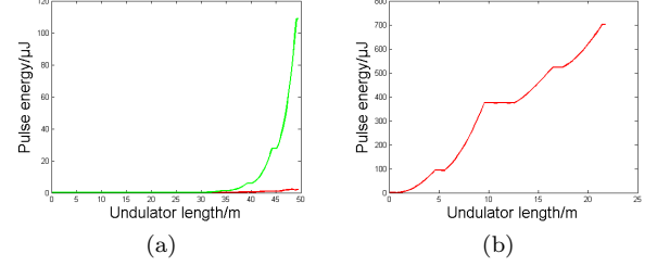
FIG. 18. The pulse energy of the linearly polarized radiation with (red) or without (green) reverse taper (a), and the pulse energy of circularly polarized radiation (b).
