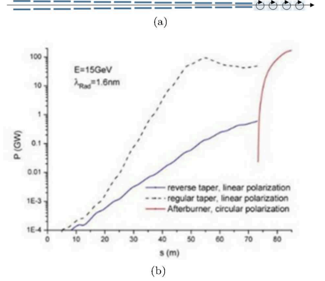
FIG. 12. Schematic of the project and the evolution of the radiation power from regular taper and reverse taper and afterburner [87], with (annexed table) the photon energy ranges generated by the UE-90 undulator by varying only the gap [88].
