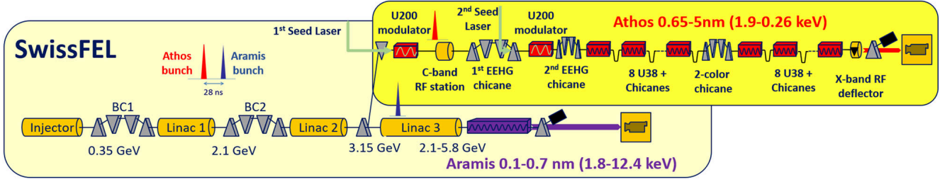
FIG. 9. The SwissFEL layout, where the injector and the three linacs are schematically represented together with the details of the two beamlines, Aramis and Athos.
