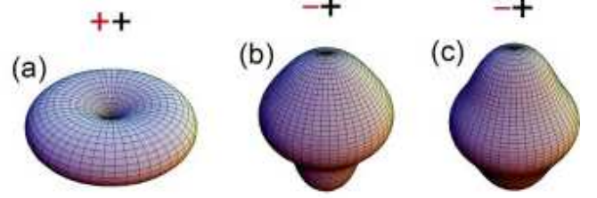
FIG. 23. PADs of the ATI of the inner 1s shell of neon for a XUV photon energy of 2 keV and an optical (NIR) photon energy of 1.5 eV. The helicity of the beams is indicated on top of each representation. (a) and (b) include the first-order non-dipole corrections, whereas panel (c) shows the PAD under the dipole approximation. The figure has been adapted from [181]
