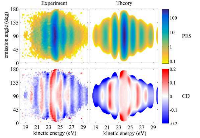
FIG. 22. Experimental (left) and theoretical (right) angle-resolved photoelectron spectra of atomic helium recorded at an XUV wavelength of 25.6 nm and a peak NIR intensity of 7.2 \times 10^{12} W/cm 2 (top) and the corresponding patterns for the angle-resolved CD (bottom). The theoretical spectra are calculated accounting for the spatial distribution of the NIR intensity, volume integrating the different values contributing to the two-color ionization process. The figure has been adapted from [181]
