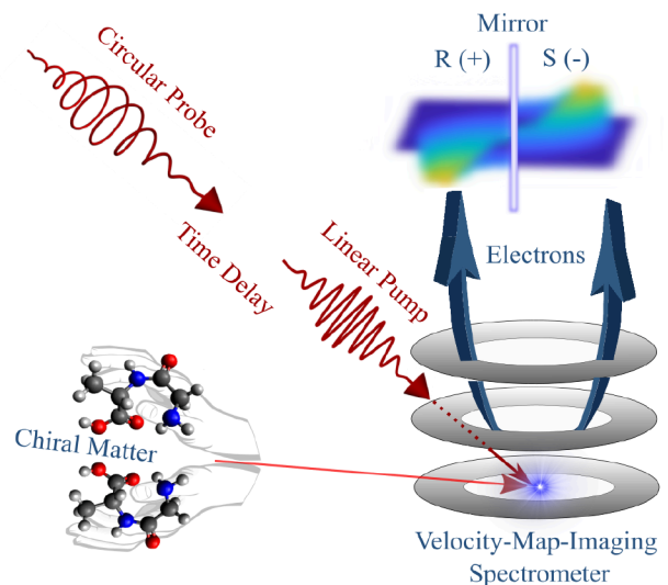
FIG. 19. Adapted figure from [107] illustrating a possible experimental scheme for pump-probe investigations of chiral systems (here glycyl-L-alanine) by VMI spectroscopy.
