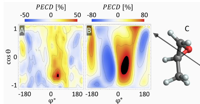
FIG. 33. Measured (panel A) and computed (panel B) differential PECDs of the O 1s-photoelectrons of S-methyloxirane with the kinetic energy of 11.5 eV as functions of the two photoelectron emission angles for the chosen molecular orientation with respect to the light propagation direction (panel C). At certain photoemission directions (indicated by black color), the measured and computed PECDs exceed the chosen upper/lower limits of the respective asymmetry scales. The figure has been adapted and reprinted with permission from [200].
