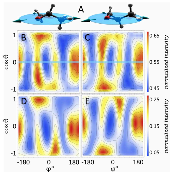
FIG. 34. A visualization of two enantiomers of methyloxirane molecule (panel A) and the respective molecular frames of reference derived from the measured asymptotic momenta of three fragments (turquoise arrows which define cyan plane for each enantiomer). Polarization-averaged angular emission distributions of the O 1s-photoelectrons with the kinetic energy of 11.5 eV, measured (panels B and C) and computed (panels D and E) for two enantiomers of methyloxirane in the frame of molecular reference. Switching between two enantiomers reflects the PA-MFPADs with respect to the cyan plane (indicated by the horizontal line in panels B and C). The figure has been adapted from [458].
