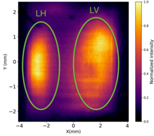
FIG. 3. Spatial profile of the two pulses produced by the cross-polarized undulator scheme with a kick in the electron-beam trajectory. Data refer to FERMI FEL-1 operated at 20.8 nm (manuscript in preparation).
