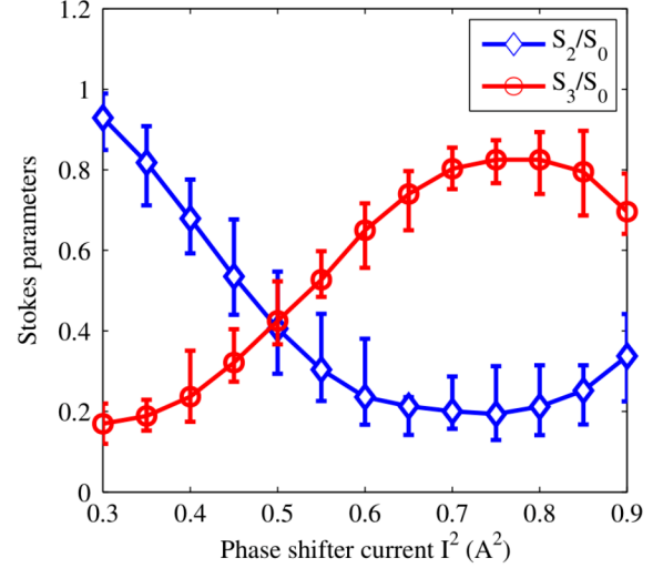
FIG. 15. The normalized Stokes parameters of coherent 523 nm radiation measured at SDUV-FEL.
