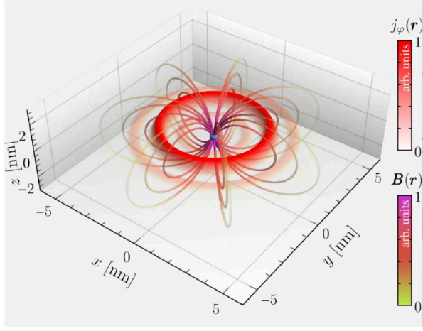
FIG. 29. Irradiating atoms by a co-propagating circularly polarized XUV laser pulse and IR vortex field carrying OAM induces in a He atom a circular unidirectional charge Rydberg current density j_\varphi(r) . The current leads to a nano-scale localized, persistent magnetic field ( B ) around each atom. The figure has been adapted from [248].
