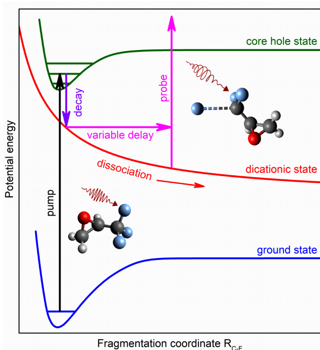
FIG. 21. A possible pump-probe experiment to investigate ultrafast chiral dynamics. The pump pulse core-excites or -ionizes a specific molecular site leaving the molecule unstable towards dissociation. Chirality of the dissociating molecule is probed with CPL via PECD. The figure has been adapted from [107].
