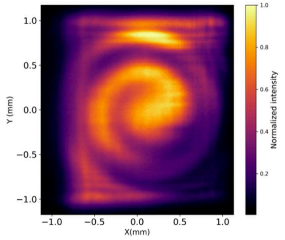
FIG. 4. FEL intensity distribution corresponding to an OAM optical mode from second harmonic emission (top) and the characteristic spiral interference pattern between the second harmonic OAM mode and the fundamental on-axis emission (bottom).
