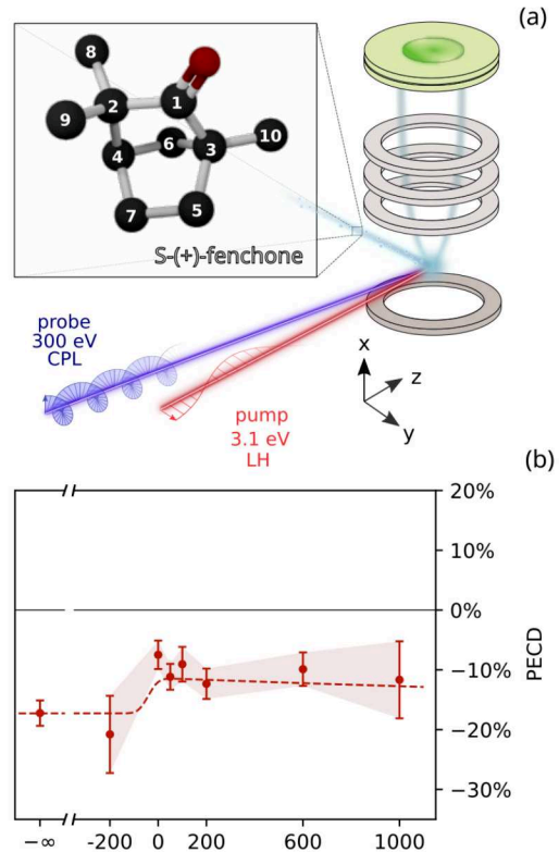
FIG. 26. (a) Experimental setup for TR-PECD. The circularly polarized XUV probe and the visible pump with linear horizontal polarization are focused quasi-collinearly in the molecular beam of S-(+)-fenchone enantiomers. The inset shows a 3D representation of the S-(+)-fenchone, where only carbon (black) and oxygen (red) atoms are shown, while hydrogen atoms are hidden for the sake of clarity. (b) Measured TR-PECD at 292.53 eV, shown with violet dots along with the error bars. The figure has been adapted from [108].
