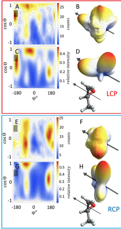
FIG. 24. Examples of measured (A,B,E,F) and computed (C,D,G,H) 3-dim. molecular-frame electron angular distributions using left circularly and right circularly polarized photons (top and bottom, respectively) for the ejection of the electron. The figure has been adapted and reprinted with permission from[200].
