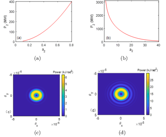
FIG. 13. Left. Emitted power from a 14 GeV electron beam entering the U-90 Apple-X afterburner after having been bunched in the main SASE3 undulator for a fixed transverse rms size of 20 \mu\text{m} (a) or a fixed bunching factor of 0.8 (b). Right. Output comparison for the beam with a bunching factor of 0.5 and a transverse size of 20 \mu\text{m} (c) and the beam with a bunching factor of 0.8 and a transverse size of 10 \mu\text{m} (d)
