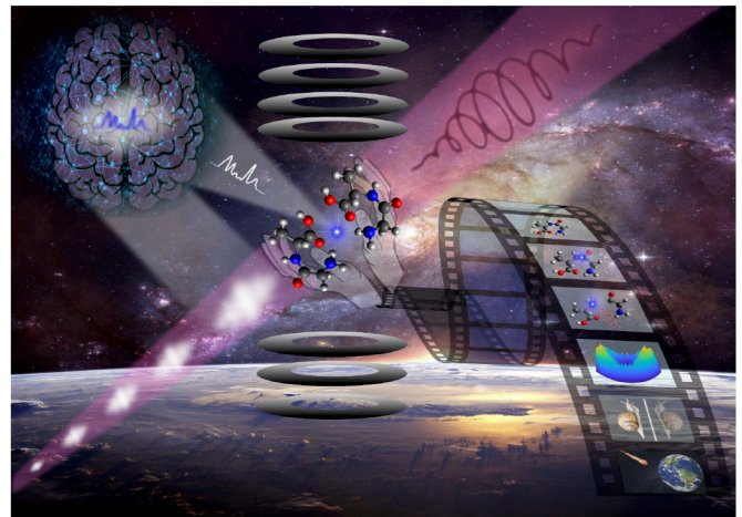
FIG. 1. Illustration of chirality science with a SASE free-electron laser. AI-based analysis reveals the time-energy and polarization structure of every ultrashort pulse. The acquired in-depth knowledge allows for site-specific observations in chiral systems and molecules (here: Glycyl-L-alanine).
