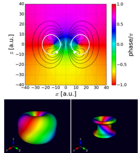
FIG. 25. Example for a chiral hydrogenic wave function \chi in form of a cut along y = 0 (top) and isosurfaces for |\chi| = 0.003 a.u. and |\chi| = 0.005 a.u., please refer to the original publication for details. The wave function's phase is indicated by the colors. The white circles in the top figure indicate the direction of the probability current in the plane y = 0 . The figure has been adapted and reprinted with permission from[202].
