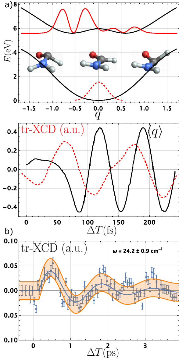
FIG. 32. a) The formamide molecule is achiral in its ground state and becomes chiral in its first excited state through pyramidalization. When pumped by circularly-polarized UV light, the nuclear wavepacket oscillates between the two enantiomers (top panel). The tr-XCD signal (middle panel, dashed, red) follows closely the nuclear wavepacket center of mass dynamics (solid, black)[172] and is a sensitive probe of the local chiral nuclear dynamics. b) tr-XCD can also be used as a local windows into chiral vibrational dynamics. In the lower panel, low-lying vibrational excitations are pumped by a UV Raman process[429] and tr-XCD is used as a local probe of chiral nuclear dynamics.
