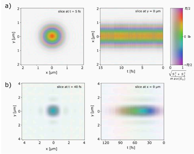
FIG. 14. Adapted from Figures 9 and 10 of [93]: Radiation polarization properties calculated for the SASE3 beamline of the European XFEL. Subplots depict radiation intensity and orientation of the polarization plane in false colors as a function of transverse coordinates and time using setup geometry, optimized for spatial , row (a) and temporal polarization shaping, row (b).
