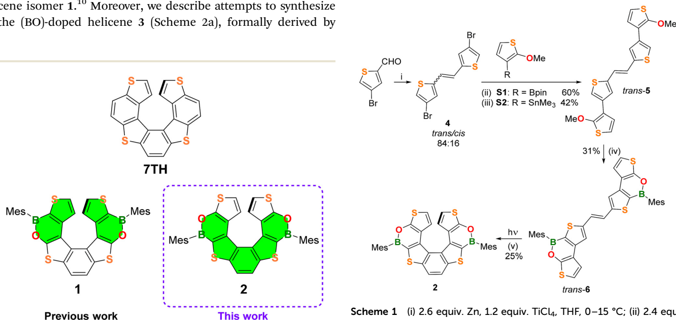
Fig. 1 Structures of the parent tetrathia[7]helicene ( 7TH ), the previously reported 1 and the newly developed (BO) 2 -helicene 2 . Mes = 2,4,6-trimethylphenyl (mesityl). The LUMO extension in the structures of 1 and 2 is highlighted in green.
