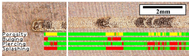
FIG. 10. Annotation of weld experiment Cu-ETP-ID3 superimposed on the weld-surface image (transformer model, wavelength data only, and truncated).
