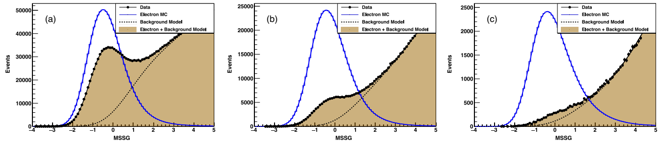
FIG. 2. The MSSG distribution for H.E.S.S. data (black data points) in three energy bands: (a) 0.3–1 TeV, (b) 1–3 TeV, and (c) > 3 TeV. The data are fitted with a parametrization of simulated electrons (blue, arb. norm.) and a parametrization of the hadronic cosmic rays (black dashed line). The combined model of electrons and hadronic background is shown as the solid black line and other area.
