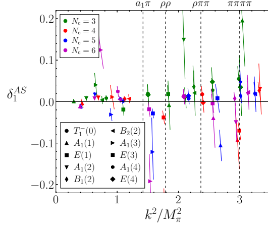
Figure 5: Preliminary results scattering phase shift in the AS channel, for N_c = 3 - 6 .
