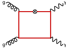
Figure 5: Sample diagram for calculating mass counter term.
