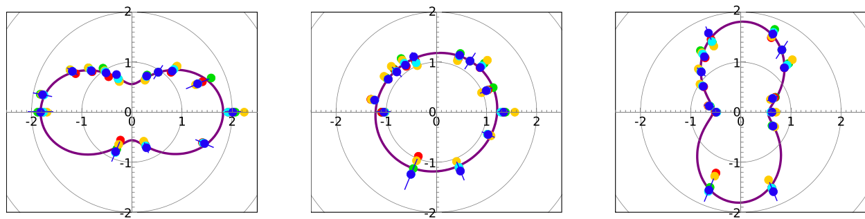
FIG. 1. Angular distribution patterns of ionization of Kr 3d at h\nu_{3rd} = 313.8 eV for different polarization modes of the FLASH2 afterburner undulator: linear horizontal (left), circular (mid), and linear vertical (right). The circles represent the measured Kr, 3d photoline intensity for each eTOF, and its corresponding angle in the dipole plane. The colors of the circles refer to different methods to determine the photoelectron signal intensity in the TOF spectrum: photoline profile fit (dark blue), raw intensity integration in an ROI around the photoline with different background definitions (light blue, yellow, and green), and photoline amplitude values (red). The purple line represents the angular distribution according to Eq. (1), with the weighted mean values for P_{lin} and \psi .
