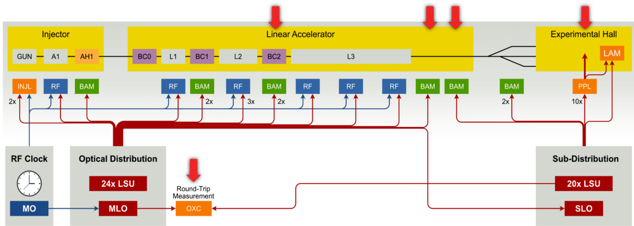
Figure 1: Sketch of the European XFEL accelerator facility and components of its pulsed optical synchronization system, with RF signal paths depicted as blue and optical fiber connections in red lines, main RF oscillator (MO), main laser oscillator (MLO), subsidiary reference laser oscillator (SLO), bunch arrival time monitors (BAM) around the bunch compressors (BC) and at the end of the linac, the "RF" re-synchronization along the accelerating stations along the linac, the laser systems of the injector (INJL) and for pump-probe experiments (PPL), and its arrival time diagnostic (LAM). The large red arrows indicate locations which are relevant for benchmark and validation experiments.
