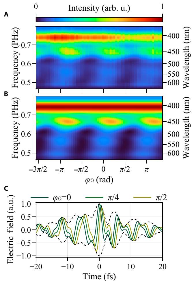
Fig. 4. Carrier-envelope phase (CEP) ( \varphi_0 ) dependence of the TRES signal. (A) Measured TRES spectrogram while varying \varphi_0 at a fixed delay and \varphi_r . The expected \pi periodicity is visible. (B) Simulated \varphi_0 scan using the pulses characterized before acquiring the data in (A). (C) E_{tot} for 3 different positions in the \varphi_0 scan. The dashed line indicates the electric field envelope.
