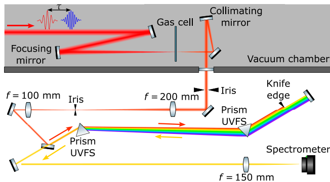
Fig. 5. Experimental setup used for the TREX measurements. Inside the vacuum chamber, the beam, consisting of 2 pulses, is focused into the gas cell where the TO signal is generated. After collimation, the beam exits the vacuum chamber and enters the spatial filtering setup used to remove the copropagating fundamentals. Here, after reducing the beam diameter with a telescope, the TO signal is spectrally dispersed by an ultraviolet (UV)-fused silica prism (UVFS). After collimation by a second prism, the fundamentals are removed with an adjustable knife edge. The signal propagates backward and is collected with a commercial spectrometer.
