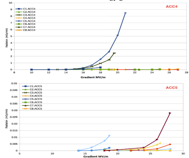
Figure 4: ACC4/5 radiation investigation at high gradient.
