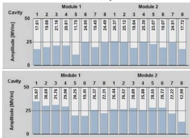
Figure 6: ACC4/5 (top, at energy gain 349.5 MeV) and ACC6/7 (bottom, at energy gain 430 MeV) gradients (peak) after RF distribution optimization.
