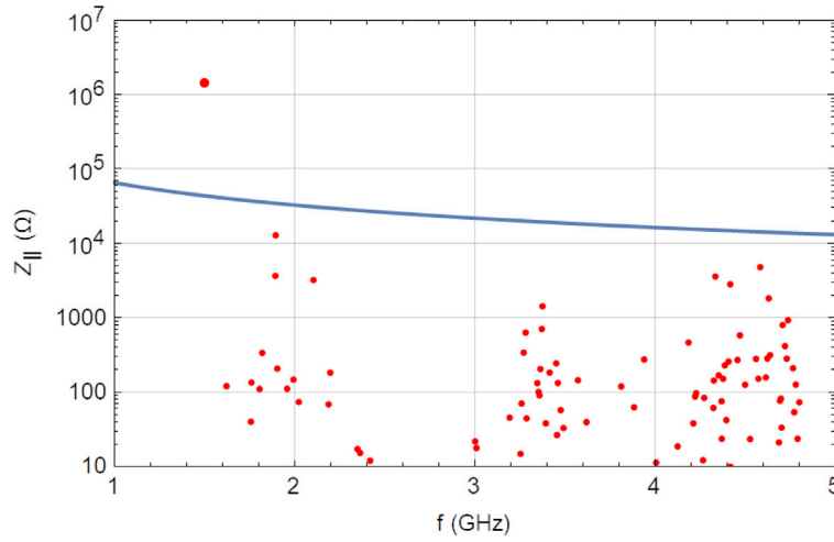
Fig. 8. Longitudinal shunt impedances of one cavity for the first 300 HOMs, including the fundamental mode. The blue curve represents the longitudinal impedance threshold Z_{||}^{\text{thresh}} for BESSY II.
