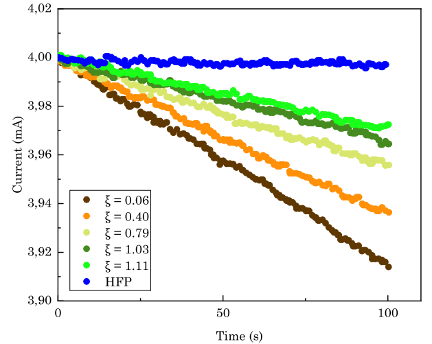
Fig. 26. Current trends for homogeneous uniform filling (HFP), and for single bunch at different harmonic voltages values, expressed as the ratio \xi .
