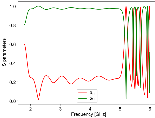
Fig. 4. S_{11} and S_{21} of the transdamper from 1.75 to 6 GHz simulated with CST MWS Studio.
