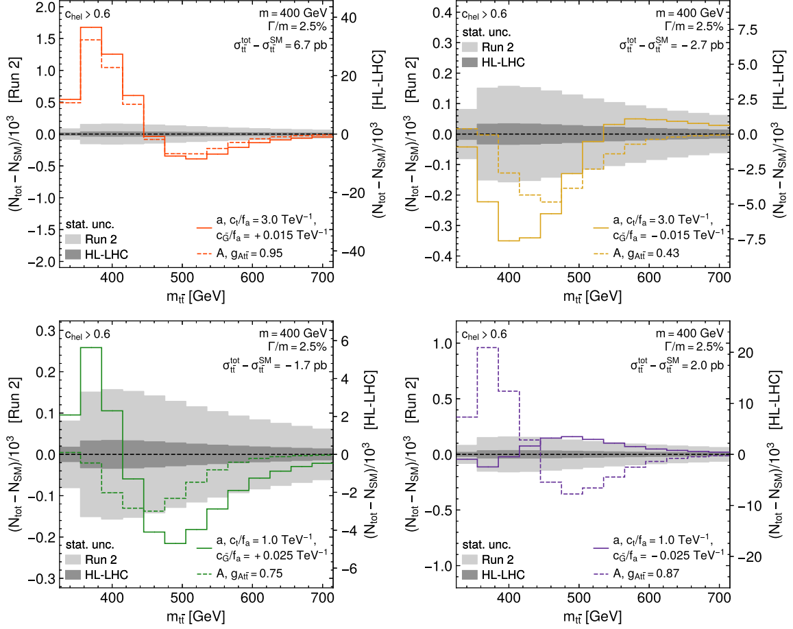
Figure 6. Differential distribution in m_{t\bar{t}} for an ALP with different values of c_{\tilde{G}} and c_t and a pseudoscalar Higgs boson with different values of g_{A t\bar{t}} , both with a mass of 400 GeV and a total width of 2.5%. The couplings c_{\tilde{G}} , c_t and g_{A t\bar{t}} are chosen in the considered benchmark scenarios such that the ALP and the pseudoscalar Higgs boson have the same integrated cross section in a given panel. Event counts are shown for integrated luminosities corresponding to Run 2 ( 138 \text{ fb}^{-1} , left axis) and the HL-LHC ( 3 \text{ ab}^{-1} , right axis). The gray bands indicate the expected statistical uncertainties on the SM background for the two integrated luminosities.
