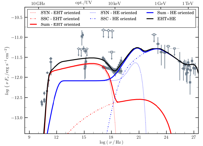
Fig. 18. Modified Model A fitted describing the BPL emission seen in the Chandra-NuSTAR X-ray spectrum.
