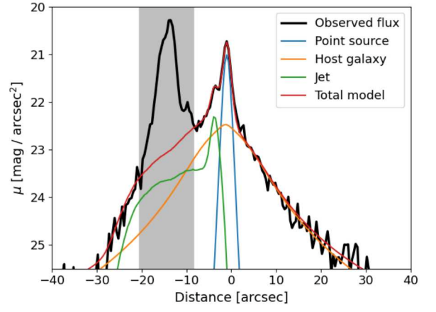
Fig. 4. AstroSat-UVIT photometric cut of the decomposition model along the jet direction. The thick black line shows the observed flux along the cut, the blue line is the central point source, the orange line is the host galaxy, the green line is the jet total flux, and the red line is the total model flux. The shaded area shows the masked out region of the jet that has a complex fine structure that cannot be accurately modelled with a simple analytical function and was therefore excluded from the decomposition to reduce the model complexity.
