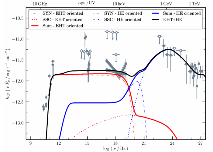
Fig. 19. Model A fitted to the observed contemporaneous broadband SED of M87 from the EHT campaign in April 2018. For each considered region (EHT and HE), the synchrotron (labeled as SYN) and synchrotron self-Compton (labeled as SSC) models as well as the summation of the two models (labeled as Sum) are reported.
