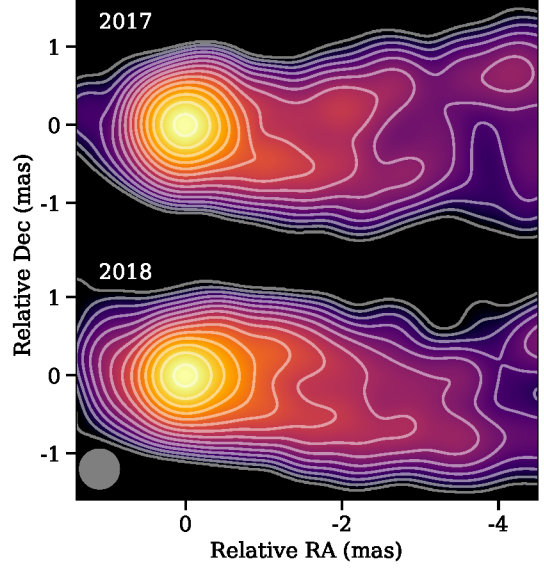
Fig. 12. M87 jet structure comparison based on yearly stacked EAVN images at 43 GHz in 2017 and 2018 (see also Cui et al. 2023 ). The restoring beam size is 0.5 mas circular Gaussian, as indicated in the bottom-left corner. The image has been rotated by -18^\circ . Contour levels are scaled as (1, 2, 4, \dots) \times C_{1st} , where C_{1st} is 1.8 mJy beam ^{-1} in 2017 and 1.3 mJy beam ^{-1} in 2018. For M87* mass M_{\text{BH}} = 6.5 \times 10^9 M_\odot ( Event Horizon Telescope Collaboration et al. 2019a ), 1 mas \approx 125 r_s \approx 0.08 pc, where r_s is the Schwarzschild radius.
