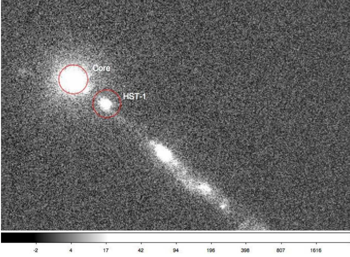
Fig. 3. Hubble Space Telescope image of M87 at 2359.7Å with the host galaxy subtracted. The core and HST-1 are indicated; the distance between the features is 1.00 \pm 0.05 , and the pixel size is 0.0248 .
