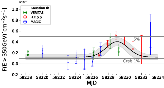
Fig. 9. Flux measurements of M87 above 350 GeV with 1\sigma uncertainties obtained with H.E.S.S., MAGIC, and VERITAS during the coordinated MWL campaign in 2018. The solid and semi-transparent colours represent the original data and scaled (with cross-normalisation factors) data, respectively. The black curve and shaded region represent the best Gaussian fit and 1\sigma error to the original flux points. The grey lines indicate the percentage of the Crab Nebula's flux level from integrating its SED in the same energy range. The SED of the Crab Nebula is obtained by fitting VERITAS's six years of observations (Meagher & VERITAS Collaboration 2015). For flux points with significance less than 2\sigma , upper limits are given in Table C.14.
