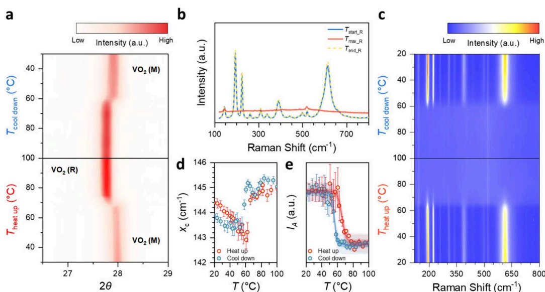
Figure 2. IMT characterization of VO 2 thin film. (a) In situ temperature-dependent GIXRD measurement zoomed in near 2\theta = 28^\circ region. The peak shown belongs to the (011) plane of VO 2 (M) at low temperature while the (110) plane of VO 2 (R) at high temperature. (b) Raman spectra at low and high temperature. (c) Temperature-dependent Raman measurement. The peak at \sim 520 cm -1 , which remains almost unaltered, is the signal from the SiO 2 /Si substrate. Lorentz fitting analysis for (d) the peak position shift and (e) the peak area as peak intensity at \sim 144.5 cm -1 as a function of temperature.
