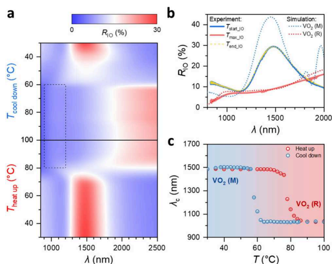
Figure 5. Switchable PBG of VO_2 IO PhC. (a) Reflection spectra R_{IO} during a heat-up and following cool-down measurement. (b) Experimental R_{IO} and simulated R_{IO} at high and low temperatures. The experimental results for T_{start\_IO} and T_{end\_IO} overlap. The small peak in the 900–1200 nm region of the curve marked as T_{max\_IO} in (b) is highlighted in the roughly corresponding region with a black dashed box in (a). The oscillation in the simulated spectrum of the VO_2 (M) phase results from Fabry–Perot interference. (c) The Bragg peak position \lambda_c as a function of temperature, showing a switch function adapted to the external temperature. The Bragg peak position \lambda_c shifts from about 1.49 \mu\text{m} below the IMT transition temperature to about 1.03 \mu\text{m} above the IMT transition temperature.
