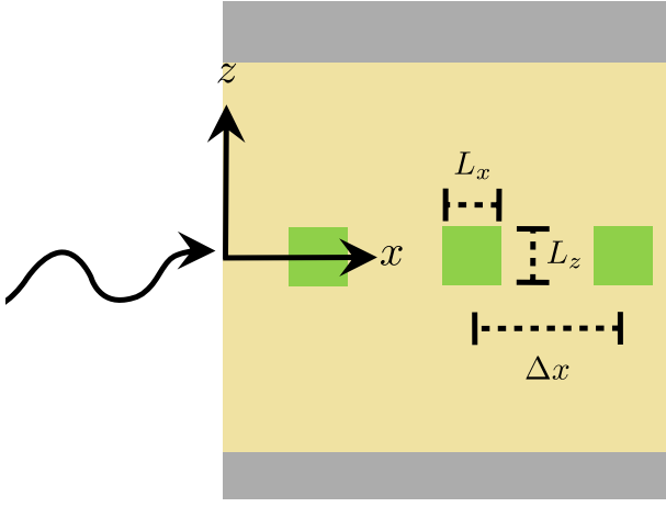
FIG. 2. Front coupling geometry, with resonant layer split into micro-strips with extent L_x, L_z , and spacing \Delta x .
