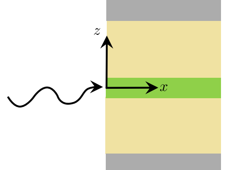
FIG. 1. Overview of scattering geometry. The waveguide is formed by a stack of dielectric layers in the z axis, while the incident beam propagates along the x axis. The field is sufficiently well collimated that it is uniform along y , allowing us to consider a two dimensional problem in the xz plane.
