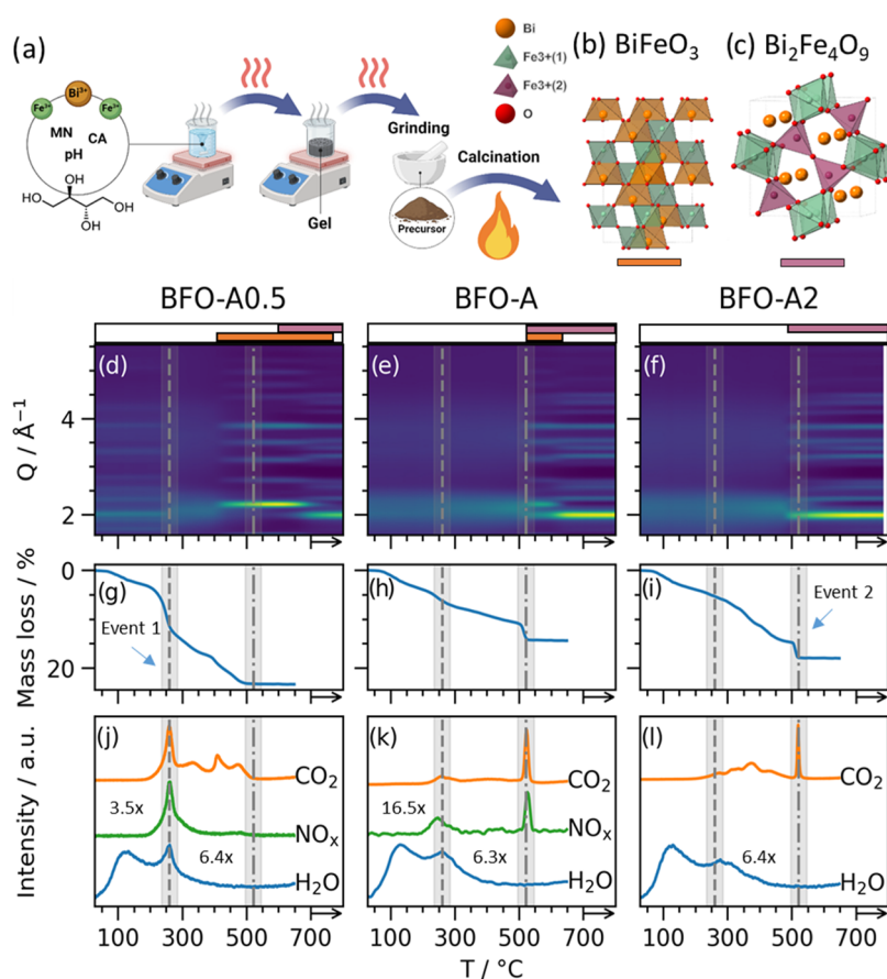
Figure 1. Synthesis and formation pathways of \text{BiFeO}_3 and \text{Bi}_2\text{Fe}_4\text{O}_9 . (a) Schematic representation of the sol–gel synthesis employed in this study; varied parameters are the pH (acidic, neutral, basic) and molar metal nitrate (MN) to the complexing agent (CA) ratio. Structures of (b) perovskite-type \text{BiFeO}_3 and (c) mullite-type \text{Bi}_2\text{Fe}_4\text{O}_9 . In situ total scattering patterns from room temperature to 700^\circ\text{C} for (d) BFO-A0.5 (MN/CA 1:0.375), (e) BFO-A (MN/CA 1:0.75), and (f) BFO-A2 (MN/CA 1:1.5) synthesized in acidic conditions (orange bars: \text{BiFeO}_3 , pink bars: \text{Bi}_2\text{Fe}_4\text{O}_9 ). Evolution of the scale factors (Figure S3) and exemplary PDF fits (Figure S2) are displayed in the Supporting Information. Corresponding (g–i) mass losses and (j–l) \text{H}_2\text{O} , \text{CO}_2 , and \text{NO}_x evolution during calcination from room temperature to 650^\circ\text{C} , as determined by TGA–MS. The dot–dashed lines highlight the breakdown of the crystalline precursor in sample BFO-A0.5 (Event 1) and crystallization of \text{Bi}_2\text{Fe}_4\text{O}_9 in BFO-A2 (Event 2). Note the different magnifications for the gas releases.
