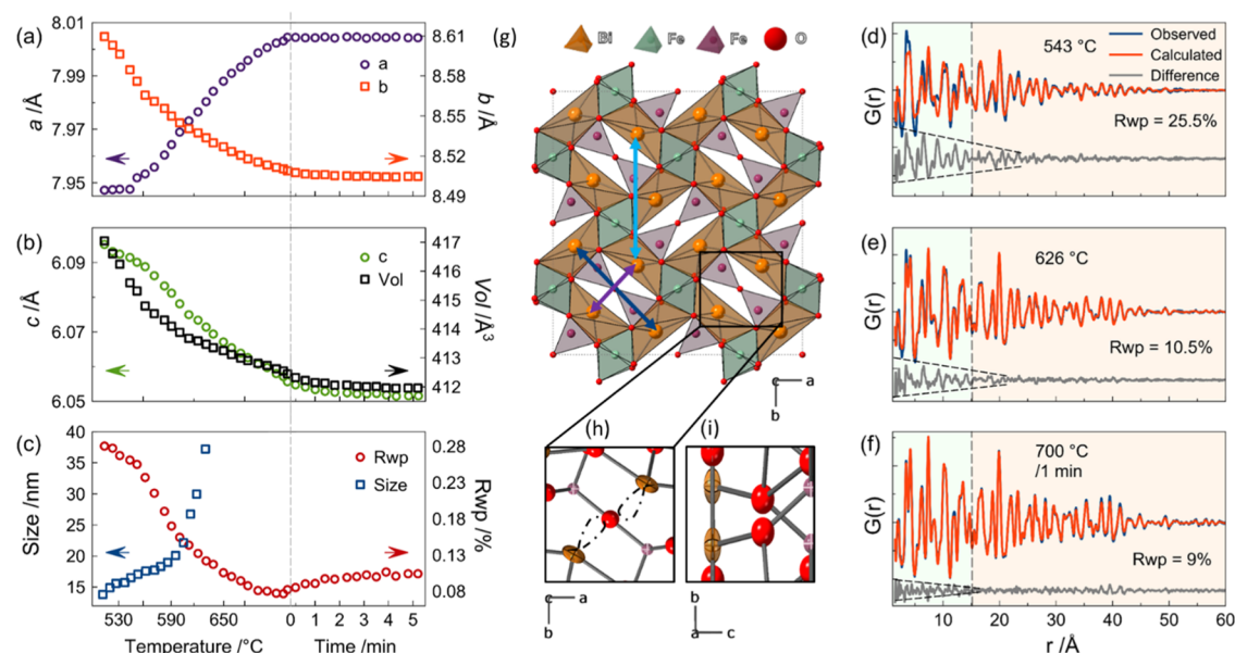
Figure 4. Temperature-dependent evolution of (a) a and b , (b) c and cell volume, and (c) crystallite size and R_{\text{wp}} during the growth of \text{Bi}_2\text{Fe}_4\text{O}_9 determined by refinements of pair distribution functions (PDF). Of note, for temperatures higher than 629 °C, the crystallites grow too big to be reliably refined, and this parameter was discarded in further refinements. Exemplary refinements of PDF data collected at (d) 543 °C, (e) 626 °C, and (f) 1 min @ 700 °C. The dot–dashed lines are guides to the eye for the local structural distortion correlation length. (g) 2 \times 2 supercell of the mullite-type \text{Bi}_2\text{Fe}_4\text{O}_9 structure with arrows indicating relevant Bi–Bi pair distances. (h, i) Thermal ellipsoids of Bi in the (h) ab -plane and (i) bc -plane. The dashed line in panel (h) serves as a guide for the eye for the expression of the 6s^2 lone electron pair of \text{Bi}^{3+} .
