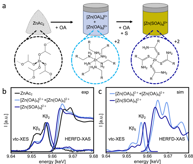
Figure 1. Identifying Zn coordination by HERFD-XAS analysis. (a) Schematics of the reaction pathway from \text{Zn}(\text{Ac})_2 precursor (black dashed circle) to a tetrahedral [\text{Zn}(\text{SOA})_4]^{2+} complex, (dark blue), which undergoes an intermediate step: a mixture of tetrahedral [\text{Zn}(\text{OA})_4]^{2+} (60%) and octahedral [\text{Zn}(\text{OA})_6]^{2+} (40%) complexes (light blue). The four and six oleylamine chains in the mixed complexes are replaced by four of their corresponding thioamide derivatives upon the addition of sulfur to the mixture. (b) Comparison of experimental HERFD-XAS and vtc-XES spectra of \text{Zn}(\text{Ac})_2 (black line), \text{Zn}(\text{Ac})_2 dissolved in oleylamine (light blue solid line) forming a mixture of [\text{Zn}(\text{OA})_4]^{2+} and [\text{Zn}(\text{OA})_6]^{2+} , and \text{Zn}(\text{Ac})_2 dissolved in oleylamine with sulfur (dark blue solid line), resulting in the [\text{Zn}(\text{SOA})_4]^{2+} complex. (c) Theoretical XAS and vtc-XES spectra obtained using DFT calculations of the proposed tetrahedral [\text{Zn}(\text{OA})_4]^{2+} mixed with octahedral [\text{Zn}(\text{OA})_6]^{2+} complexes at the ratio 60:40, and the [\text{Zn}(\text{SOA})_4]^{2+} complex. Peaks in vtc-XES spectra above the Fermi level are described by multielectron excitations in the literature. 46,47 ( R = (\text{CH}_2)_7(\text{HC} = \text{CH})(\text{CH}_2)_7(\text{CH}_3) ).
