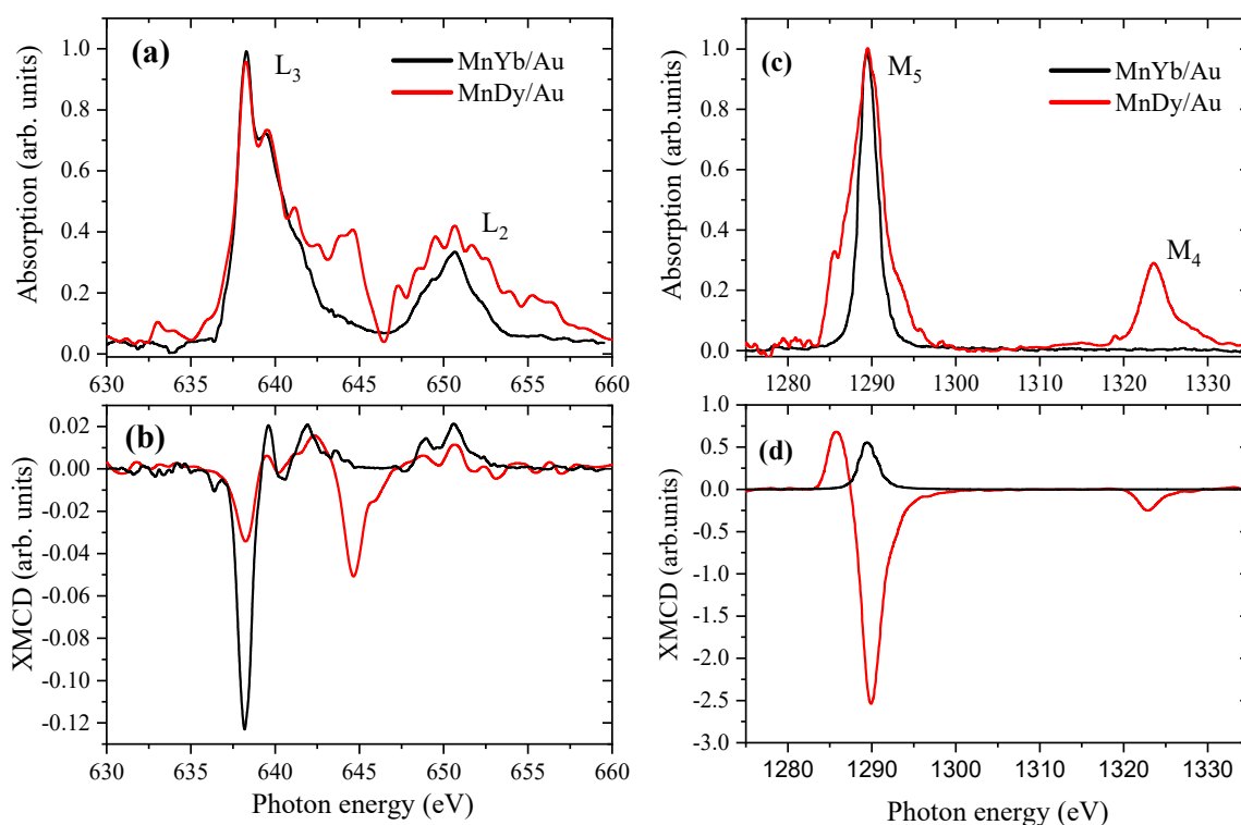
Figure 13. Comparison of Mn L_{2,3} -edges (left panel) and Dy M_{4,5} -edges (right panel) XAS (a,c) and XMCD (b,d) spectra of \{Mn^{II}_3Mn^{IV}Dy^{III}_3\} and \{Mn^{II}_3Mn^{IV}Yb^{III}_3\} coordination complexes deposited on the Au substrate.
