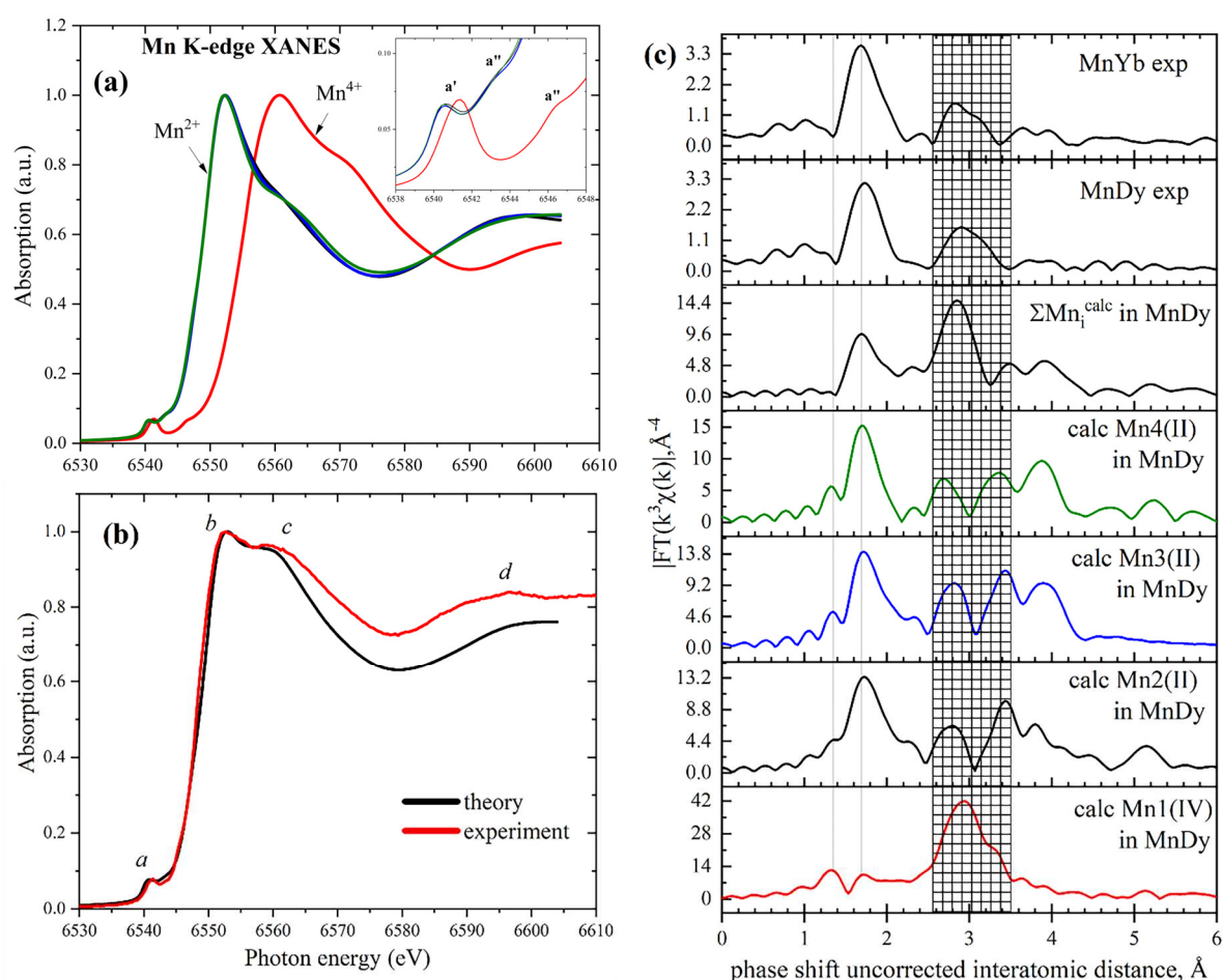
Figure 2. (a) Theoretical Mn K-edge XANES spectra of four manganese atoms of the \{\text{Mn}^{\text{II}}_3\text{Mn}^{\text{IV}}\text{Dy}^{\text{III}}_3\} coordination complex; (b) comparison of the experimental Mn K-edge spectrum with a total spectrum of all four nonequivalent Mn atoms; (c) Fourier transforms of Mn K-edge k^3 weighed EXAFS. Mn1...Mn4 are the numbers of the Mn atoms according to Figure 1.
