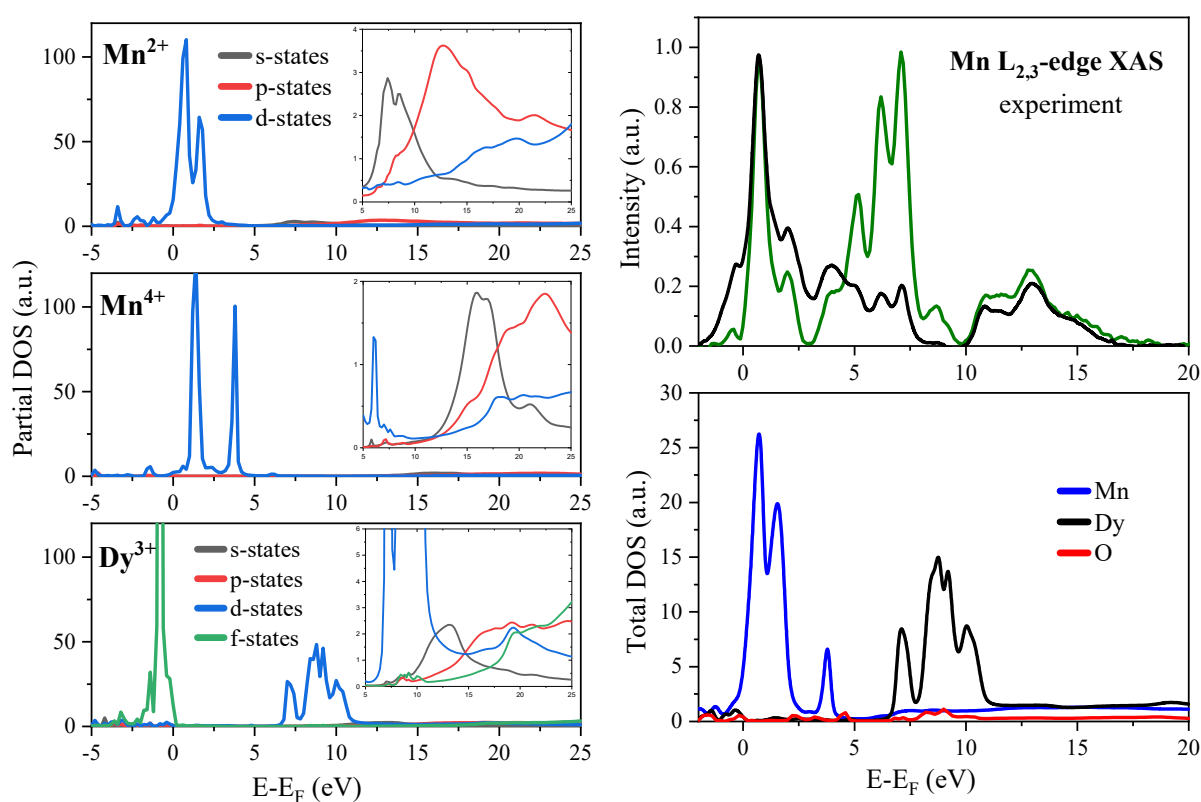
Figure 4. (left): partial density of states for Mn 2+ and Mn 4+ atoms ((top) and (middle) panels) and Dy atoms ((bottom) panel); (right): the experimental Mn L_{2,3} XAS spectra of the \{\text{Mn}^{\text{II}}_3\text{Mn}^{\text{IV}}\text{Dy}^{\text{III}}_3\} coordination complex measured at the PEAXIS (green line) and 4IDC (black line) beamlines (top) and the calculated total density of states spectra for Mn and Dy atoms (bottom). The Fermi level is set at 0 eV.
