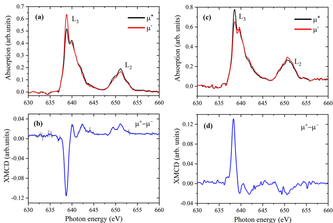
Figure 12. Mn L_{2,3} -edge XAS and XMCD of the \{Mn^{II}_3Mn^{IV}Yb^{III}_3\} coordination complexes deposited on the Au substrate measured at the magnetic field of 5T (left panel) and -5T (right panel). Labels (a,c) and (b,d) correspond to the XAS and XMCD spectra, respectively.
