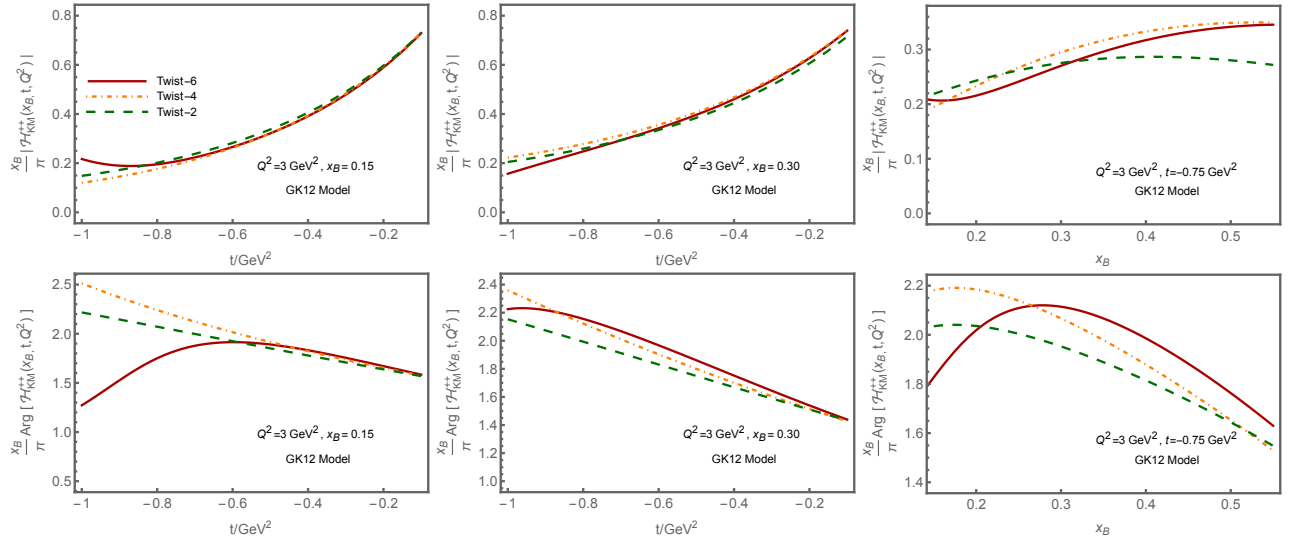
Figure 2. Kinematic power corrections to the absolute value and phase of the KM Compton Form Factor \mathcal{H}_{\text{KM}}^{++}(x_B, t, Q^2) .
