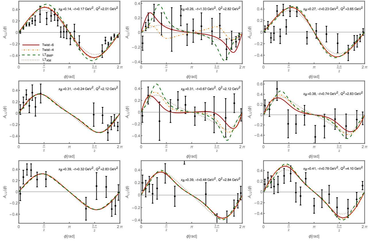
Figure 6. Beam spin asymmetries from Jefferson Lab CLAS12 10.6 GeV data set [42] (selected data sets).
