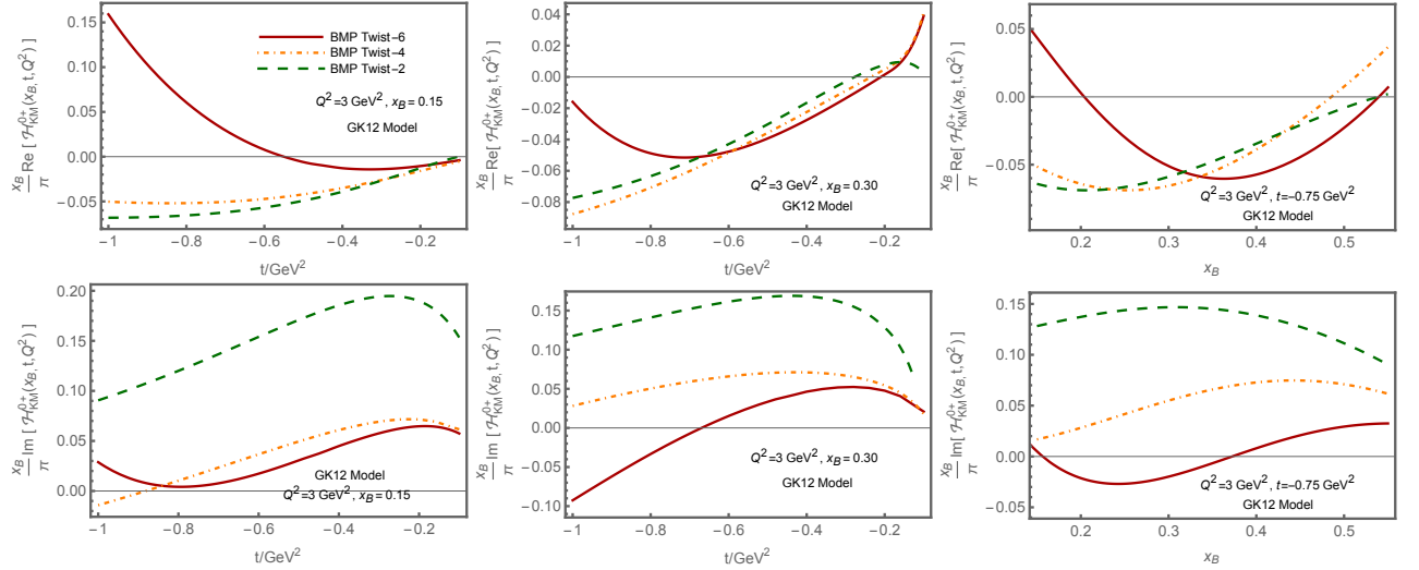
Figure 4. Real (upper panels) and imaginary (lower panels) parts of the helicity-flip KM Compton Form Factor \mathcal{H}_{\text{KM}}^{0+}(x_B, t, Q^2) .
