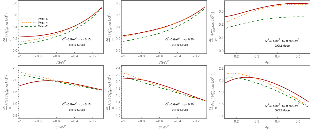
Figure 1. Kinematic power corrections to the absolute value and phase of the BMP Compton Form Factor \mathcal{H}_{\text{BMP}}^{++}(x_B, t, Q^2) .
