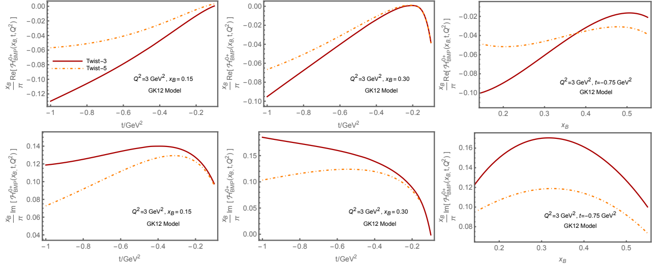
Figure 3. Real (upper panels) and imaginary (lower panels) parts of the helicity-flip BMP Compton Form Factor \mathcal{H}_{\text{BMP}}^{0+}(x_B, t, Q^2) .
