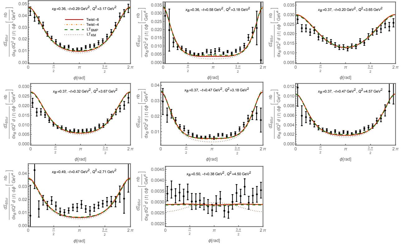
Figure 5. Spin-averaged cross sections from Jefferson Lab HallA [32] (selected data sets).
