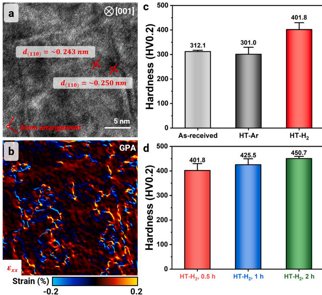
Fig. 6. (a) Image-corrected high-resolution TEM (HR-TEM) image of the HT- H_2 specimen along [001] zone axis. (b) Map of strain distribution ( \epsilon_{xx} ) of the HT- H_2 specimen determined by geometric phase analysis (GPA) of HR-TEM image from the same area in (a). (c) Hardness (HV0.2) of as-received, HT-Ar, and HT- H_2 specimens after the heat treatment (hardness measurements were conducted one week after the heat treatment). (d) Hardness (HV0.2) evolution of specimens treated in H_2 at 500 °C for 0.5 h (HT- H_2 ), 1 h (HT- H_2 -1h), and 2 h (HT- H_2 -2h).
