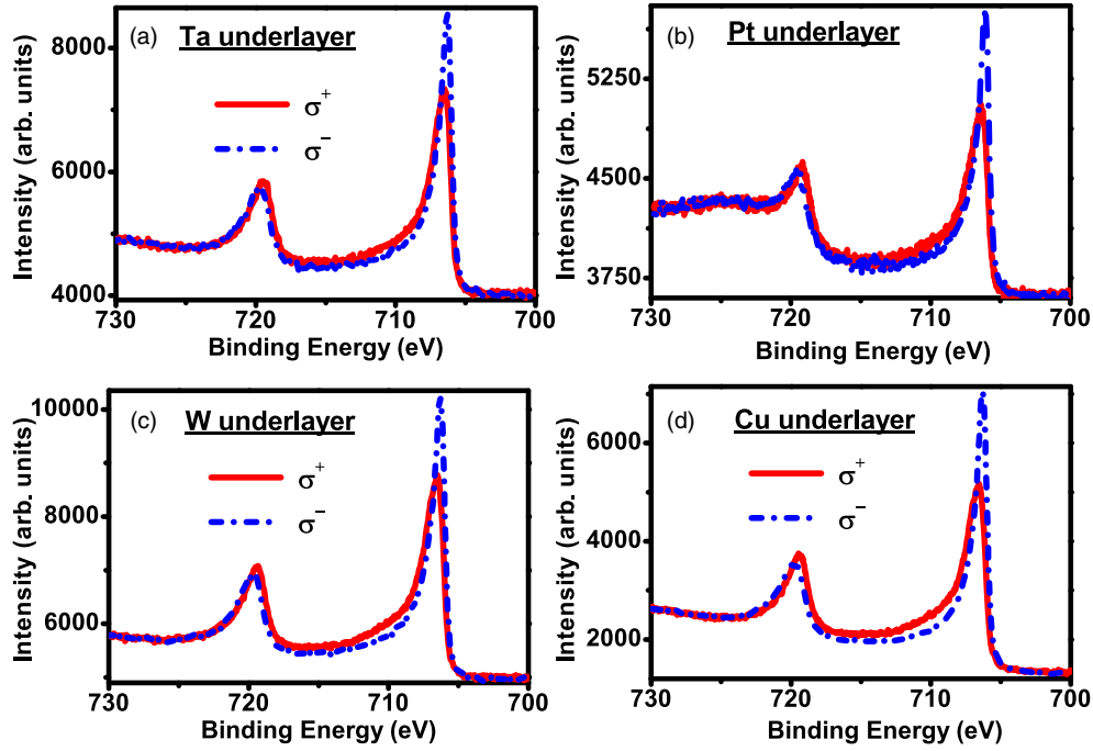
FIG. 1. Dichroic Fe-2p HAXPES intensity ( I^{\sigma^{\pm}} ) versus binding energy data recorded using right \sigma^+ and left \sigma^- polarized X-ray photons recorded on (a) CoFeB/Ta, (b) CoFeB/Pt, (c) CoFeB/W, and (d) CoFeB/Cu heterostructures.
