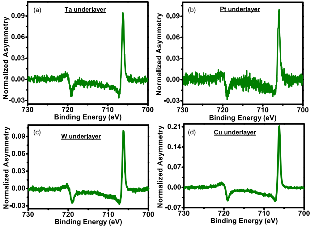
FIG. 2. Calculated Fe-2p dichroic asymmetry ((I^{\sigma^-} - I^{\sigma^+}) / (I^{\sigma^+} + I^{\sigma^-})) for (a) CoFeB/Ta, (b) CoFeB/Pt, (c) CoFeB/W, and (d) CoFeB/Cu heterostructures.
