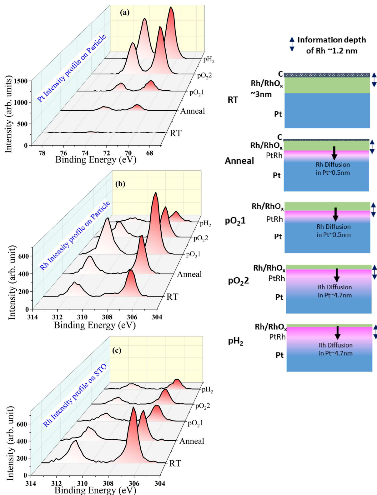
Figure 2. Intensity distribution of (a) Pt 4f spectra on top of the Pt particle, (b) Rh 3d spectra on top of the Pt particle, and (c) in the vicinity on STO extracted from the XPEEM images at each experimental condition. The sketch on the right side is a schematic representation of the Rh behavior on the Pt particle at each experimental condition.
