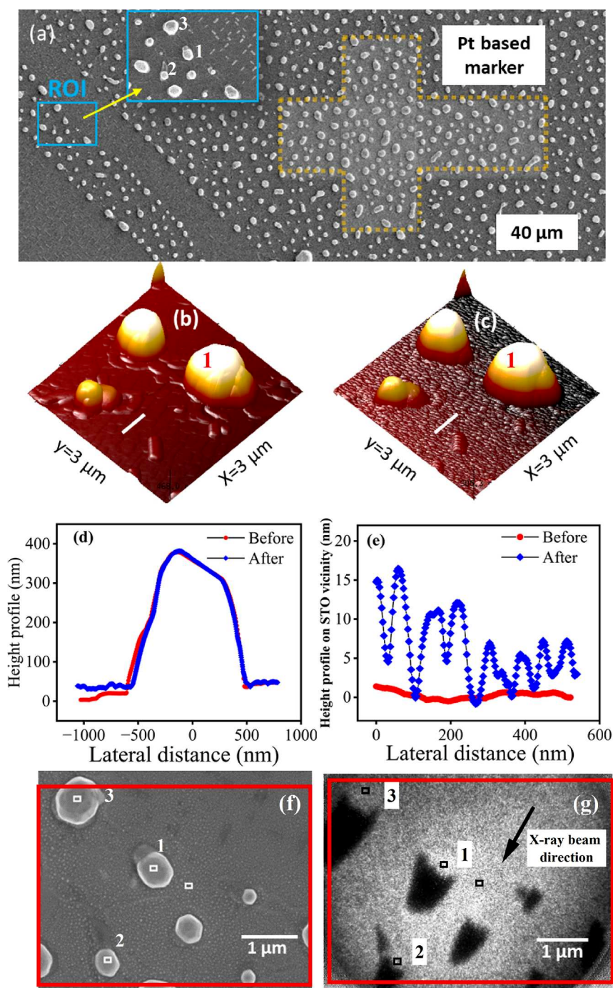
Figure 1. (a) SEM micrograph of the Pt–Rh core–shell nanoparticles' arrangement on the STO substrate. The small square in the SEM image represents the ROI for in-depth analysis, which was relocated by the Pt-based marker (dotted line). The inset shows a larger view of the selected ROI. (b,c) Comparison of the AFM topography of the ROI before and after the in situ experiment. (d) AFM height profiles of particle 1, labeled in Figure 1b,c, and (e) the Rh height distribution in the vicinity on the STO before and after the in situ experiment. (f) SEM image after the in situ experiment and (g) Rh XPEEM image at a photon energy of 390 eV of the corresponding ROI at RT. The arrow shows the direction of the X-ray beam and the red frames indicate the registered common image region.
