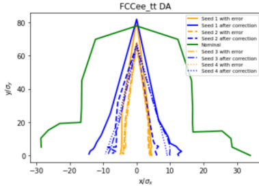
Figure 3: Arc quads subjected to 20 μm alignment errors.
