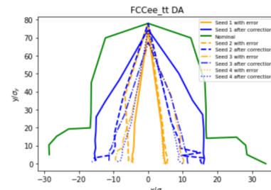
Figure 2: Arc quads subjected to 10\mu\text{m} alignment errors.
