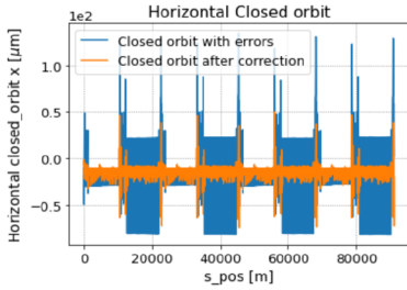
Figure 4: Horizontal closed orbit with 10 μm alignment errors before and after orbit correction.
