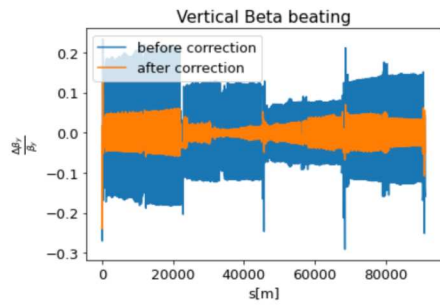
Figure 6: Arc quads subjected to 10 \mu\text{m} alignment errors.
