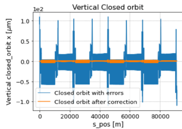
Figure 5: Vertical closed orbit with 10 μm alignment errors before and after orbit correction.
