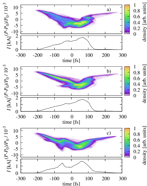
Figure 5: Longitudinal phase-space density and current profile of a bunch that is (a) unheated, (b) heated by a single laser pulse, (c) heated by two partially destructively interfering laser pulses.
