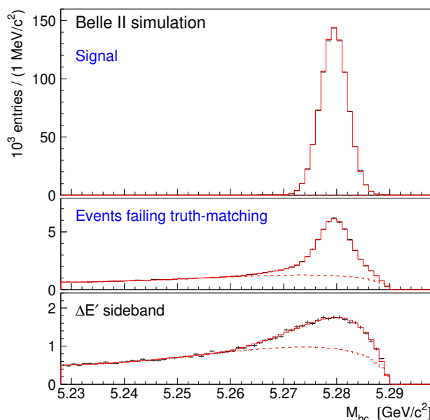
Figure 4. Distributions of M_{bc} for the simulated \Upsilon(4S) sample. The top and middle panels show truth-matched and non-truth matched candidates, respectively, while the bottom panel shows candidates in the \Delta E' sideband. The solid histogram shows the result of the simultaneous fit, and the dashed histogram shows the distribution of background events.
