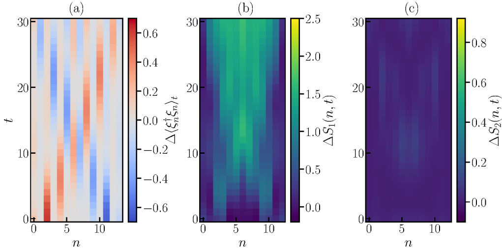
Figure 5: (a) Particle density, (b) entropy \Delta S_1(n, t) and (c) subtracted entropy \Delta S_2(n, t) for the non-interacting system with 14 sites and m = 0.8 . The initial Gaussian fermion (antifermion) wave packet is located around the site n = 2 ( n = 11 ) with the mean momentum \mu_k^c = 2\pi/N ( \mu_k^d = -2\pi/N ). Both wave packets have the same width in momentum space \sigma_k = 2\pi/N .
