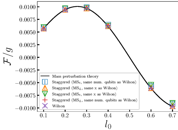
FIG. 6. Electric field density \mathcal{F}/g against l_0 for Wilson fermions and staggered fermions at m_r/g = 0.01 . The following MSE values are the mean squared error of each of the data as compared to the continuum mass perturbation theory prediction for the electric field density \mathcal{F}/g given in Eq. (20). For staggered fermions with MS t and same x (number of qubits as Wilson), the MSE is 1.041 \times 10^{-6} ( 6.16 \times 10^{-7} ), and respectively for MS L 6.143 \times 10^{-9} ( 2.617 \times 10^{-8} ). For Wilson fermions the MSE is 7.926 \times 10^{-9} . The error bars emanate from the errors in the variational algorithm to compute the relevant ground states, the extrapolation in bond dimension and in lattice spacing.
