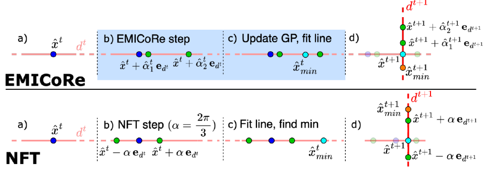
Figure 1: Illustration of EMICoRe (ours) and NFT [11] (baseline) procedures. In each step of NFT (bottom row), a) given the current best point \hat{x}^t and the direction d^t to be explored, b) next observation points are chosen in a deterministic fashion. Then, c) the minimum along the line is found by the sinusoidal function fitting to the three points, and d) the next optimization step for the new direction d^{t+1} starts from the found minimum \hat{x}^{t+1} = \hat{x}_{\min}^t . The EMICoRe procedure (top row) uses GP regression and BO in the steps highlighted by the light blue box: b) the next observation points are chosen by BO with the EMICoRe acquisition function based on the GP trained on the previous observations, and c) minimizing the predictive mean function of the updated GP with the new observations gives the best point \hat{x}_{\min}^t .
