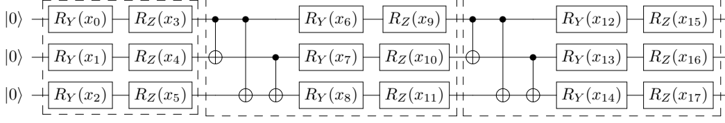
Figure 6: Illustration of Qiskit’s [43] Efficient SU(2) Circuit with default parameters for Q = 3 qubits and L = 2 layers (thus \mathbf{x} \in [0, 2\pi)^{18} ). Each dashed box indicates a layer of the ansatz circuit. The quantum computation proceeds from left to right with an initial ansatz of the form |0\rangle^{\otimes Q} . Each horizontal line corresponds to a quantum wire representing one qubit. The symbols on the wires correspond to gate operations on the respective qubits, starting with two parametrized rotational gates R_Y and R_Z acting on the qubits in the initial 0-th layer. Then, each of the following layers is composed of one block of CNOT gates and two rotational gates acting on each qubit.
