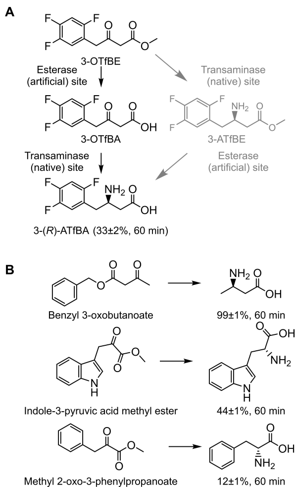
Scheme 2. Schematic representation the one-pot reaction products for converting a set of \beta -keto esters by TR_2E_2 . A) Schematic representation of the two possible routes for converting 3-OTfBE into 3-ATfBA. As shown in the figure, the preferential route is the production of 3-ATfBA via hydrolysis of 3-OTfBE to 3-OTfBA, which then yields (R)-3-ATfBA, and not via formation of 3-ATfBE (gray color). B) Schematic representation of one-pot synthesis of amino acids from a set of \beta -keto esters. The conversion, determined by HPLC for all substrates, at 60 min is shown. The figure was created using ChemDraw 18.2.
