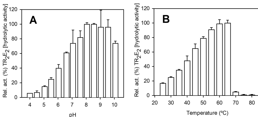
Figure 3. Optimal parameters for assessing the hydrolytic activity of purified TR 2 E 2 . A) TR 2 E 2 activity toward 3-OTfBE at different pH values. Reaction conditions: [protein]: 31 μM; [3-OTfBE]: 7.2 mM; pH: 50 mM Britton–Robinson (BR) buffer with a pH ranging from 3 to 11; reaction volume: 100 μL; and T: 30 °C. B) TR 2 E 2 activity toward 3-OTfBE at different temperatures. Reaction conditions: [protein]: 31 μM; [3-OTfBE]: 7.2 mM; T: 25–80 °C; pH: 100 mM K 2 HPO 4 buffer, pH 7.5; and reaction volume: 100 μL. In both cases, the reactions were performed in triplicate and were incubated for 15 min at 750 rpm, after which 300 μL of a solution composed of acetonitrile, H 2 O and formic acid (10:10:0.6) were added to stop the reaction. Substrate depletion was detected using HPLC. The figure was created using SigmaPlot 14.0 software.
