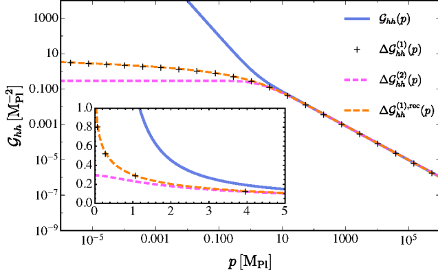
Figure 8. Comparison of \Delta\mathcal{G}_{hh}^{(1),\text{rec}} (dashed orange line) reconstructed in this work with that in [12], \Delta\mathcal{G}_{hh}^{(1)} (black plus markers). The difference propagator \Delta\mathcal{G}_{hh}^{(1),\text{rec}} has been computed by plugging \rho_h^{\text{cont}} in the spectral representation (31).
