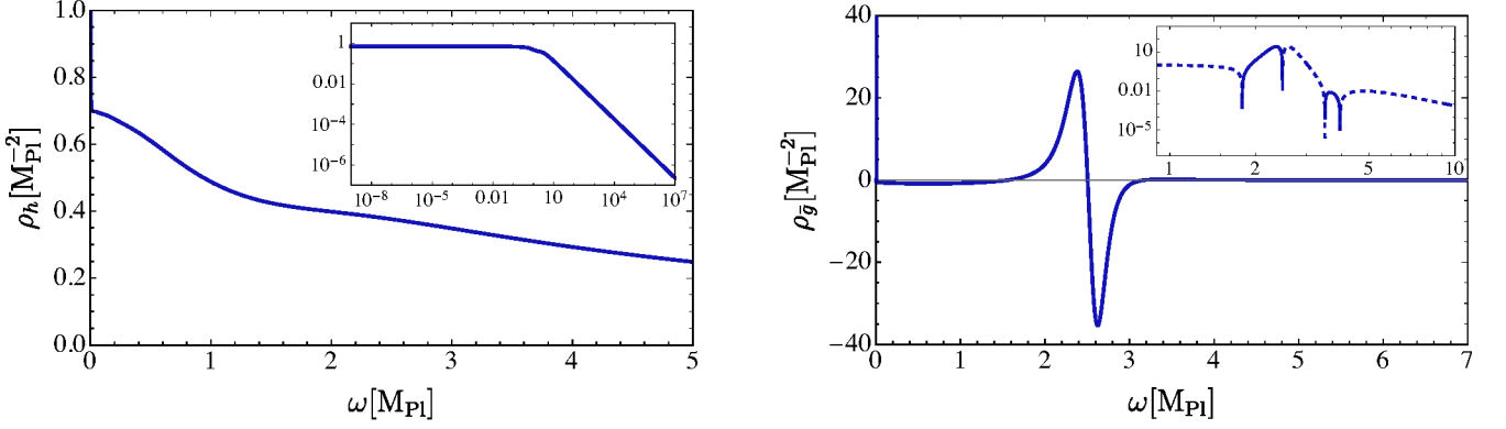
Figure 3. The spectral function of the fluctuation (left panel) and background (right panel) graviton fields. Both feature a Dirac delta peak at \omega = 0 (massless graviton) and a smooth multi-particle continuum for positive frequencies. The background spectral function contains positive and negative parts and has a vanishing spectral weight. The latter feature is better displayed in the inset plot in the top-right corner, in which we show the absolute value. The solid and dashed lines in the inlay show the positive and negative parts of the spectral function, respectively.
