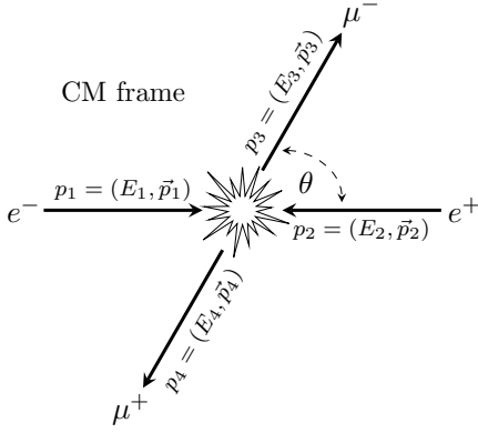
Figure 7. Kinematics of e^- e^+ \rightarrow \mu^- \mu^+ in the centre-of-mass frame. Since the particles are all on-shell, p_i = \sqrt{E^2 - m_e^2} and p_f = \sqrt{E^2 - m_\mu^2} .
