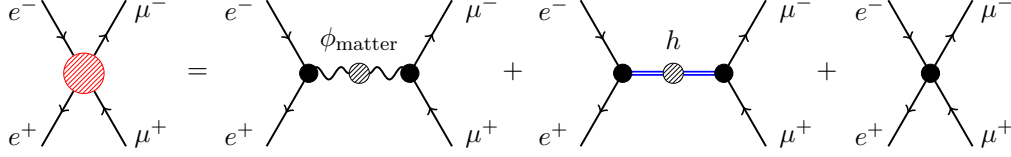
Figure 1. Electron-positron to muon-antimuon scattering in terms of diagrams with full 1PI vertices. The scattering process is mediated by matter propagators (first diagram) and by a graviton propagator (second diagram) as well as the contact term (third diagram). Full black circles indicate full 1PI vertices and dashed circles indicate full 1PI propagators.
