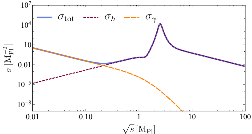
Figure 4. Total (solid blue line) and partial contributions to the e^+e^- \rightarrow \mu^+\mu^- cross-section taking into account the effects from asymptotically safe quantum gravity. The dashed orange and dotted purple lines depict the photon-mediated and graviton-mediated contributions.
