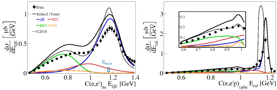
Figure 8: (left) The 1.159 GeV C(e,e')_{0\pi} cross-section plotted as a function of the reconstructed energy E_{QE} and (right) the 1.159 GeV C(e,e'p)_{1p0\pi} cross-section plotted as a function of the reconstructed energy E_{cal} , for data (black points), GENIE SuSAv2 (solid black curve) and GENIE G2018 (dotted black curve). The colored lines show the contributions of different processes to the GENIE SuSAv2 cross-section: QE (blue), MEC (red), RES (green) and DIS (orange). Error bars show the 68% ( 1\sigma ) confidence limits for the statistical and point-to-point systematic uncertainties added in quadrature. Error bars are not shown when they are smaller than the size of the data point. Normalization uncertainty of 3% not shown. Figure adapted from [1138].
