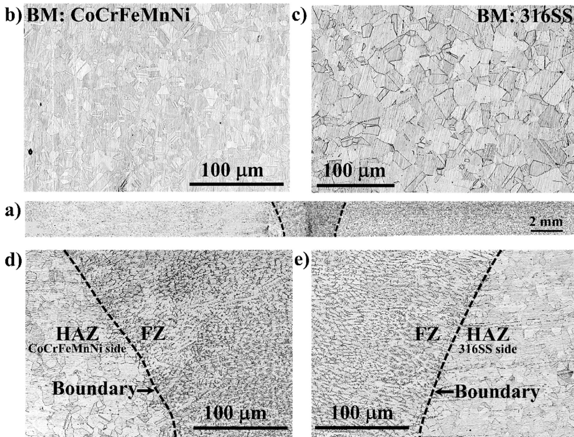
Fig. 2. a) a cross-sectional view of dissimilar GTA-welded CoCrFeMnNi HEA to 316 stainless steel; b)-e) are close-up views of optical/electron microscopy for the CoCrFeMnNi HEA BM, 316 stainless BM, the boundary of HAZ/FZ near the CoCrFeMnNi HEA side and HAZ near the 316 stainless steel, respectively.
