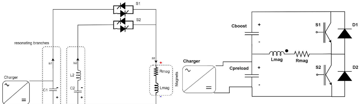
Fig. 6.7: Full wave (left) and switched (right) discontinued resonance principles
