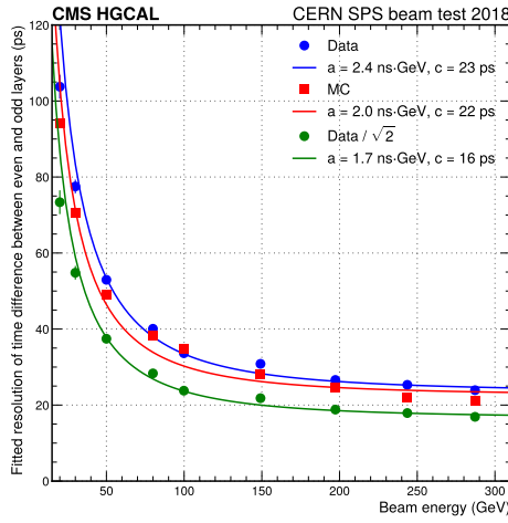
Figure 10. Resolution of the event-by-event difference between the time of positron half-showers computed with only even layers and only odd layers separately, as obtained for beam data (blue) and simulated Monte Carlo (MC) data (red). The green markers correspond to beam data resolutions divided by \sqrt{2} , and are an estimate of the performance expected if all the layers were used for the shower time estimation. These measurements are not affected by the jitter between MCP and HGCal, as discussed in the text.
