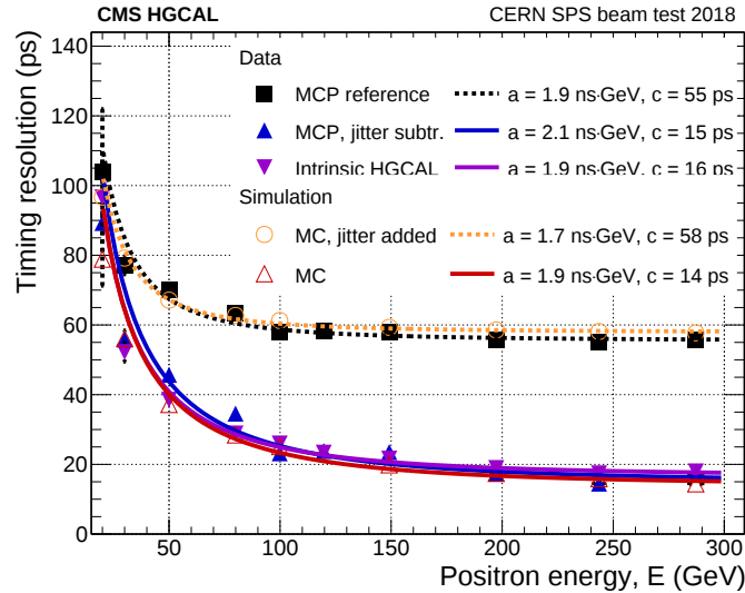
Figure 13. Comparison of the HGICAL prototype timing resolution for positron showers in data and simulated samples. For data, the resolution is measured for all layers using the MCP as a reference (black squares) as well as using only half the layers with respect to the other half and assuming they have identical resolution (purple triangles). Other measurements in the figure allow to cross-check and confirm the hypothesis that a global jitter between the MCP and HGICAL systems was present in the data.
