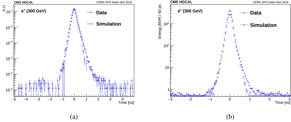
Figure 12. For the hits used in the reconstruction of the same 300 GeV positron showers, (a) time distribution of the fraction of hits and (b) the average and standard deviation of the energy of hits as a function of their calibrated time. Beam data in full markers and simulated data in empty markers.
