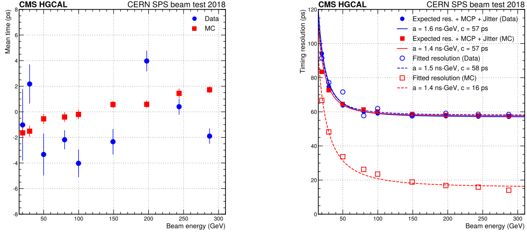
(a) Average shower time showing an accuracy better than 10 ps across the full range of energies probed.
