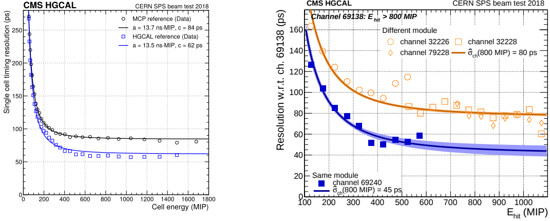
(a) Single-channel timing performance taking the MCP (black circles) or the HGICAL shower measurement (blue squares) as reference.
