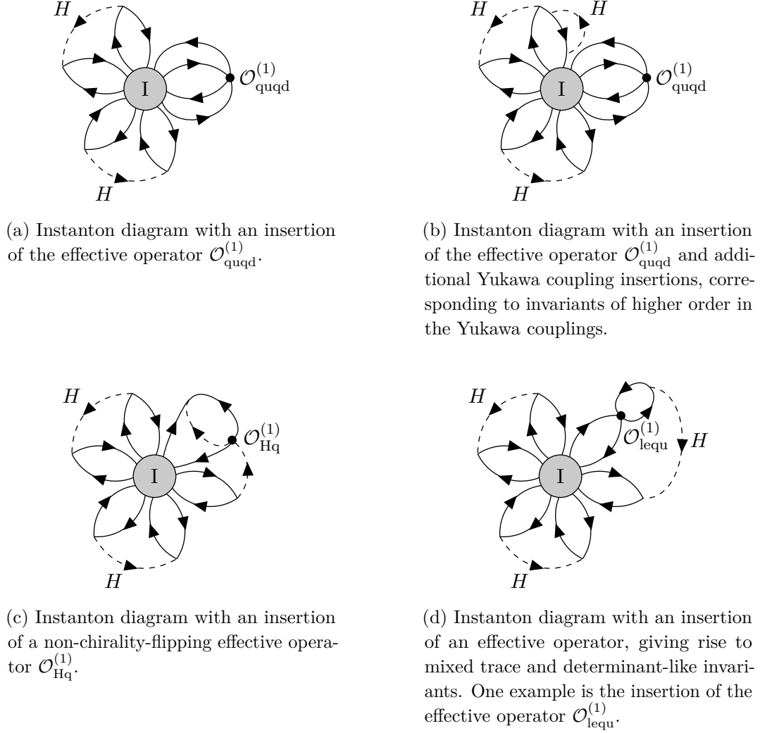
Figure 1. Examples of instanton diagrams corresponding to invariants discussed in the text. Here, the gray blob depicts the instanton background that the fermions (solid lines) are coupled to. The fermion lines are closed via Yukawa interactions with the Higgs (dashed lines).
