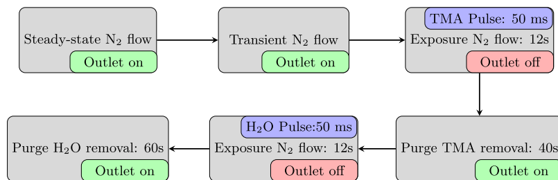
Figure 2. Flowchart for simulating precursors distributions of one full cycle of Al 2 O 3 deposition. N 2 is used as a carrier and purging gas. The outlet resembles the stop valve which connects the ALD chamber with the vacuum pump. Outlet is On when the stop valve is open and the chamber is pumped, while outlet is OFF during nonpumping, namely, exposure stage.
