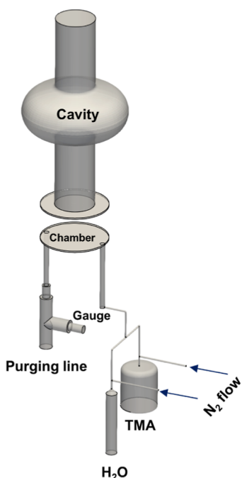
Figure 1. 3D computational domain in the digital twin which is based on the used homemade ALD setup. The system consists of two precursors (TMA and H 2 O) inlets and one outlet for exhaust. Reaction chamber for thin film samples and cavity on the top of the chamber: here, the whole cavity is considered as a reaction chamber.
