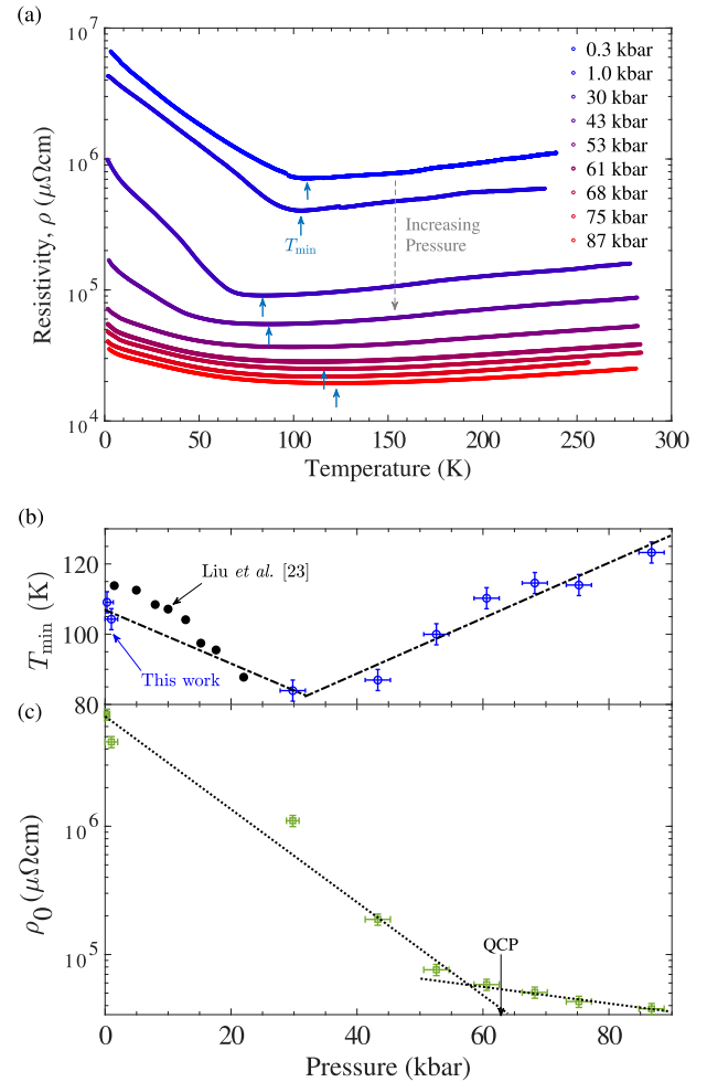
Fig. 4 Resistivity vs temperature at high pressures. a Resistivity vs temperature for increasing applied pressures, plotted on a logarithmic y-axis. The temperature position of the resistivity minimum, T_{\min} , is marked with arrows. b Values of T_{\min} plotted against applied pressure, blue open circles. Data from the work of Liu et al. 33 are overlaid as closed black circles. c Resistivity extrapolated (via a quadratic fit below 8 K) to T = 0 K plotted against pressure. Note that the vertical axis is logarithmic. Dotted lines are intended as guides to the eye, highlighting a change of behavior around 60 kbar, close to the Ir AIAO QCP. Error bars show the uncertainties in determining pressure (see Methods) and in the values of T_{\min} and \rho_0 .
