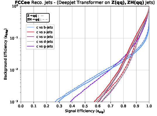
(b) charm tagging
