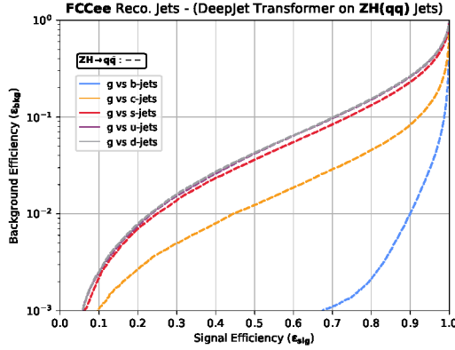
(e) gluon tagging
