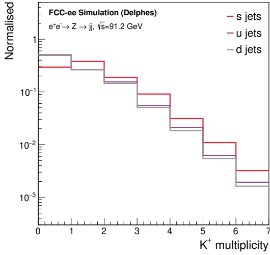
(c) Kaon multiplicities.
