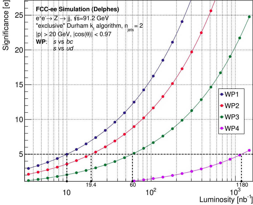
Figure 10: Discovery Significance vs Luminosity for the four working points corresponding to Table 8. The points noted by the x axis intersecting with the dashed vertical lines are the luminosities required at the four respective working points to achieve the canonical discovery significance of 5\sigma .
