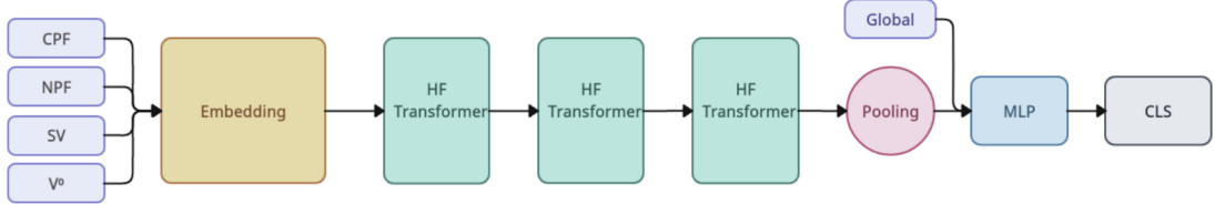
Figure 4: Schematic structure of DeepJetTransformer model.
