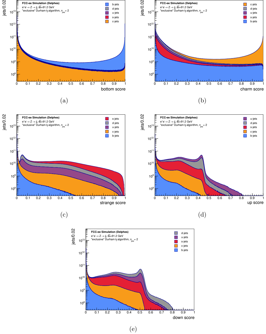
Figure 5: The softmaxed classifier outputs ( S_i ) of the five output nodes of DeepJetTransformer trained with clustered jets of e^+e^- \rightarrow Z \rightarrow q\bar{q} events at \sqrt{s} = 91.2 GeV. The contributions of different MC flavours have been displayed.
