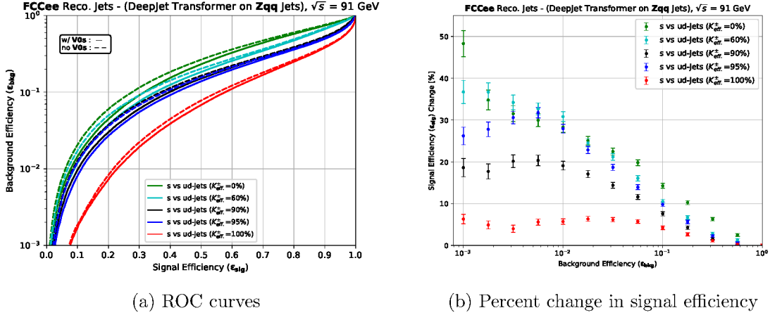
Figure 8: The dependence of strange jet tagging performance on the inclusion of V^0 s and charged Kaon identification scenarios. (a) ROC curves for s vs ud tagging at the Z resonance at \sqrt{s} = 91.2 GeV. Solid lines represent results with the inclusion of V^0 s, while dashed lines show the results without them. (b) Percent change in signal efficiency ( \epsilon_{sig} ) with the inclusion of V^0 s for s vs ud tagging for each of the K^\pm ID scenarios listed in Table 5. The axes are swapped with respect to Figure 8a to present the percent change in signal efficiency ( \epsilon_{sig} ) as a function of 12 fixed background efficiencies ( \epsilon_{bkg} ).
