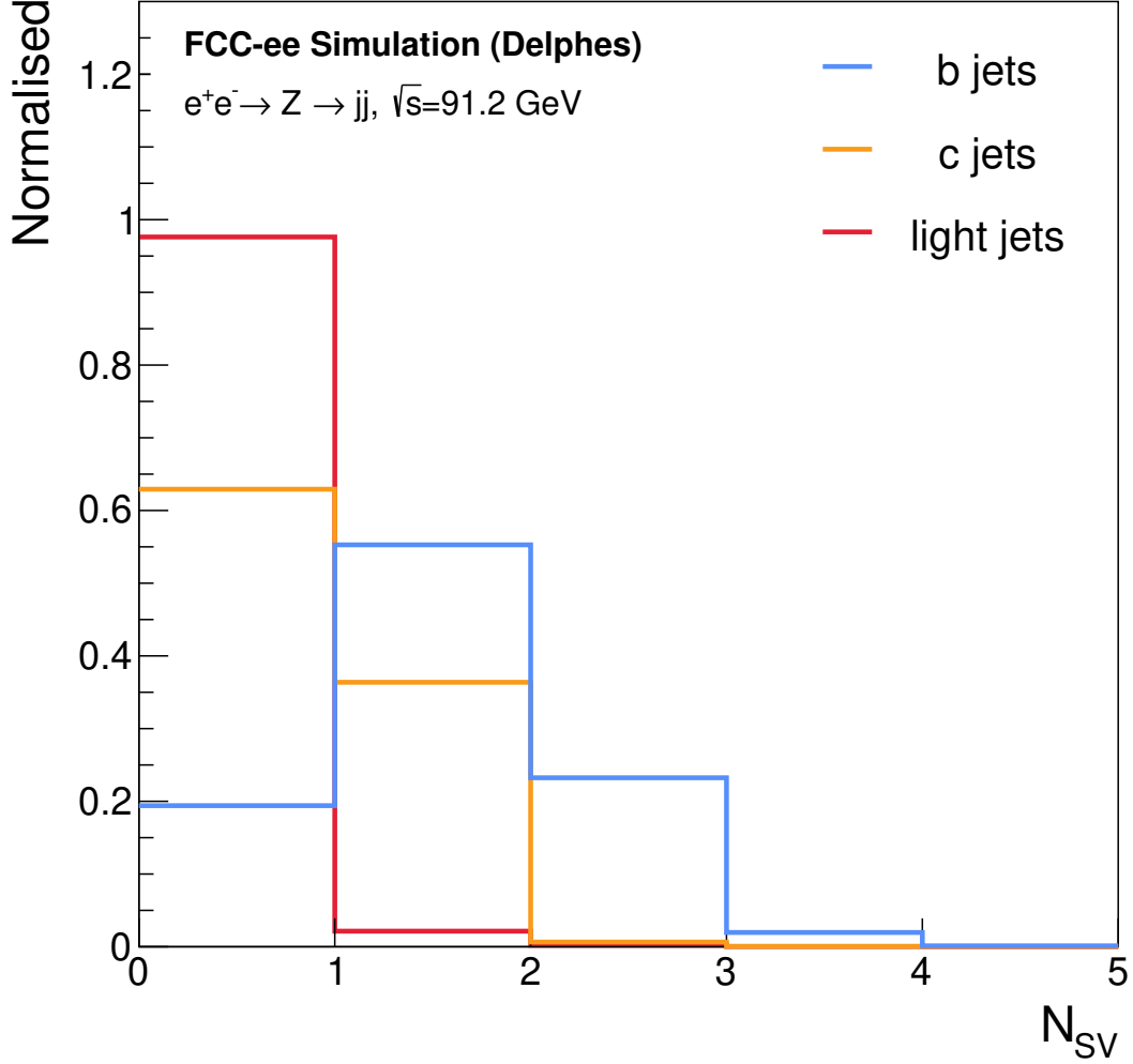
Figure 2: SV multiplicity in jets from e^+e^- \rightarrow Z \rightarrow q\bar{q} events. The term “light jets” here collectively refers to u -, d -, and s -jets.
