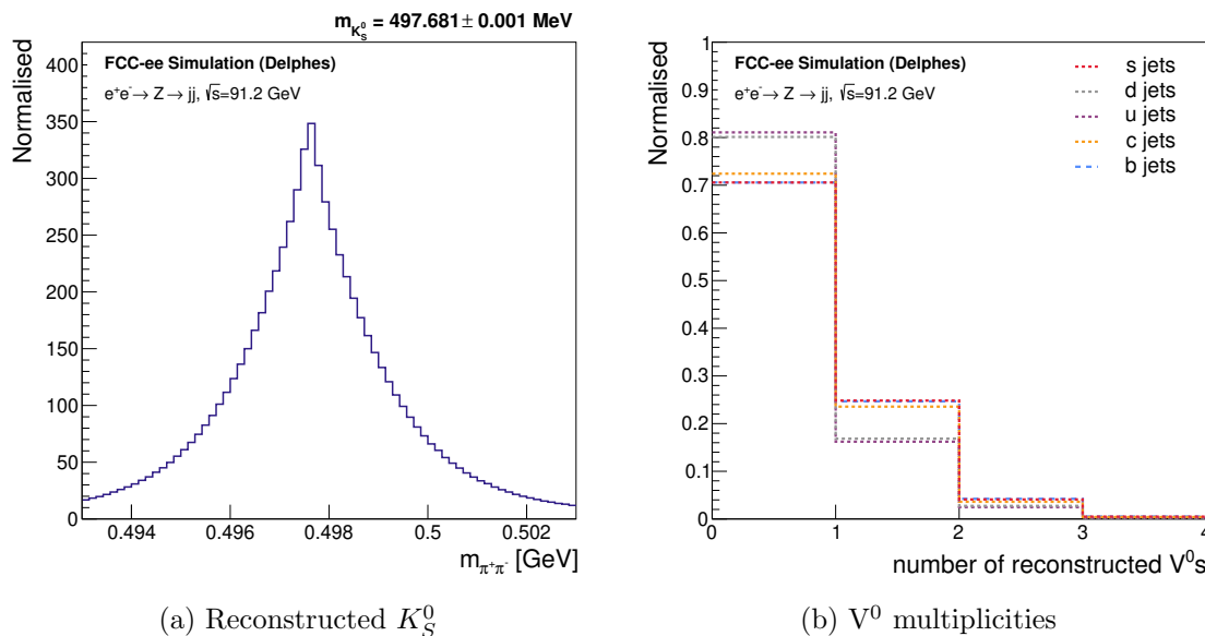
Figure 1: Performance of V^0 reconstruction. (a) Invariant mass distribution of reconstructed K_S^0 vertices. The quoted mass is the mean and the error on the mean of the distribution. (b) The reconstructed V^0 multiplicity in jets from e^+e^- \rightarrow Z \rightarrow q\bar{q} events at \sqrt{s} = 91.2 GeV, where q \equiv u, d, s, c, b . The distributions for b - and s -jets overlap almost perfectly.
