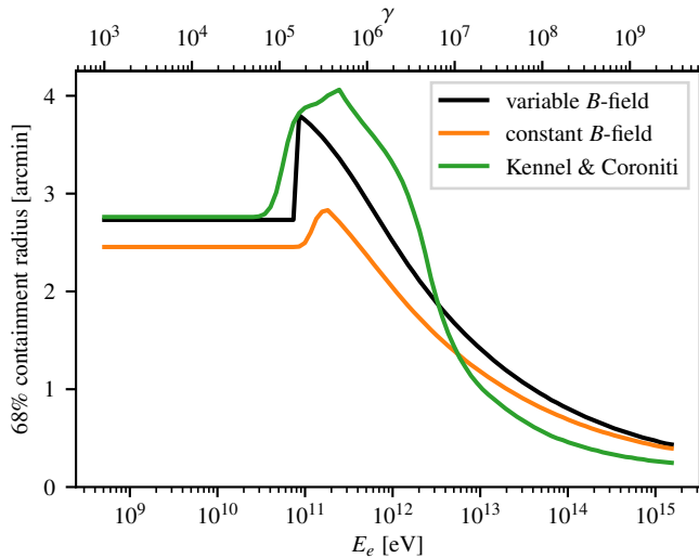
Fig. 15. Comparison of the 68% containment radii of the electron energy densities of the three models. The radio electrons dominate the low-energy part of the spectrum where the extension is not energy-dependent. The extension of the wind electrons changes with energy, following, in case of the static models, a simple power law. The spectral transition of the two distributions is shown in Fig. 8.
