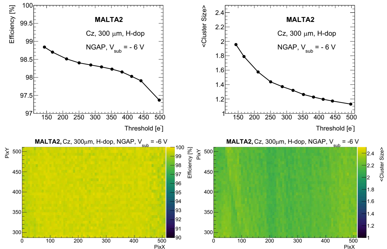
Fig. 5 Average efficiency (top left) and cluster size (top right) as a function of threshold. The bottom images show their respective 2D map at a threshold corresponding to 150 \text{ e}^- . Results are shown for a non-irradiated MALTA2 sample (Cz, NGAP, 300 \mu\text{m} thick, high doping of n^- layer) at V_{\text{sub}} = -6 \text{ V}
