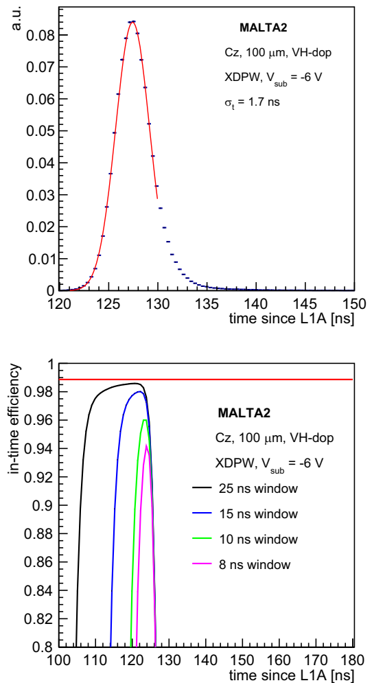
Fig. 13 Top image shows time of arrival of the leading hit in the cluster with respect to a scintillator reference. The quoted \sigma_t = 1.7 ns corresponds to the Gaussian fit to the core of the distribution. Bottom image shows in-time efficiency. Black curve corresponds to in-time efficiency within a 25 ns window, blue curve corresponds to a 15 ns windows, and the green and magenta cure represent a 10 and 8 ns window, respectively. Red line represents maximum achievable efficiency without timing constraints. Both measurements are performed on a MALTA2 sample (Cz, XDPW, very high doping n^- layer, 100 \mu\text{m} thick) at V_{\text{sub}} = -6 V. The threshold corresponds to 170 e^-
