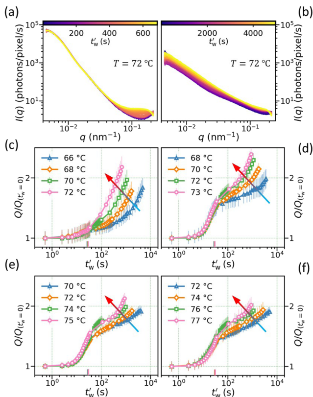
FIG. 5. Evolution of I(q) of (a) pure egg yolk and (b) y2000 at T = 72 °C. The color bar indicates the absolute waiting time t'_w from the onset of heating at 22 °C. The normalized scattering invariant Q/Q(t_w=0) as a function of t'_w for (c) yolk, (d) y500, (e) y1000, and (f) y2000. The small vertical lines close to the horizontal-axis indicate t_{\text{heating}} (time taken to reach the set temperature of 22 °C). The color of these lines matches that of data points at the same temperature. The arrows point in the direction of increasing temperatures.
