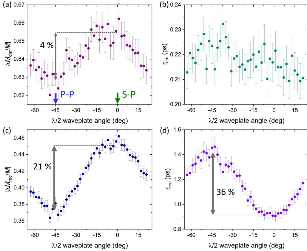
FIG. 3. Fit results of dynamics in Pt/Co/Pt: (a) demagnetization amplitude \Delta M_{\text{dm}} , (b) demagnetization time \tau_{\text{dm}} , (c) recovery amplitude \Delta M_{\text{rec}} , and (d) recovery time \tau_{\text{rec}} as a function of the pump 1 polarization direction, determined by the rotation of the half waveplate, after excitation with two pump beams. Pump 2 was always P polarized. The fluence for the two pumps was 4 mJ/cm 2 . The half waveplate position when excited in the P-P and S-P configurations is indicated in panel (a).
